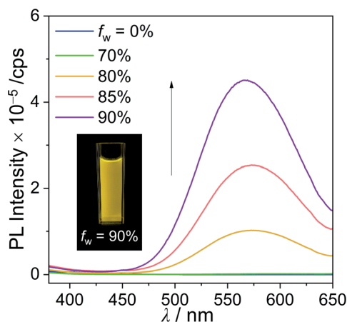
Fig. 4 PL spectra of closo-Cz ( \lambda_{\text{ex}} = 331 nm) in THF/distilled water mixtures ( 3.0 \times 10^{-5} M). The inset show the emission colour under irradiation by a hand-held UV lamp ( \lambda_{\text{ex}} = 365 nm).
