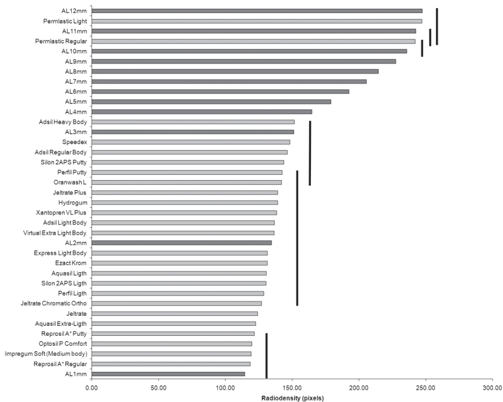
Figure 6- Comparison between materials and aluminum stepwedge. Bars not connected by the same line are statistically different by Kruskal Wallis and Dunn's Method ( p < 0.05 )
