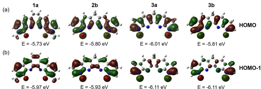
Fig. 5 (a) HOMO and (b) HOMO–1 of ligands 1a , 2b , 3a and 3b and their energies.
