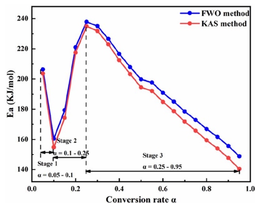
Fig. 6 Relationship between reaction activation energy and conversion rate of phosphate tailings.
