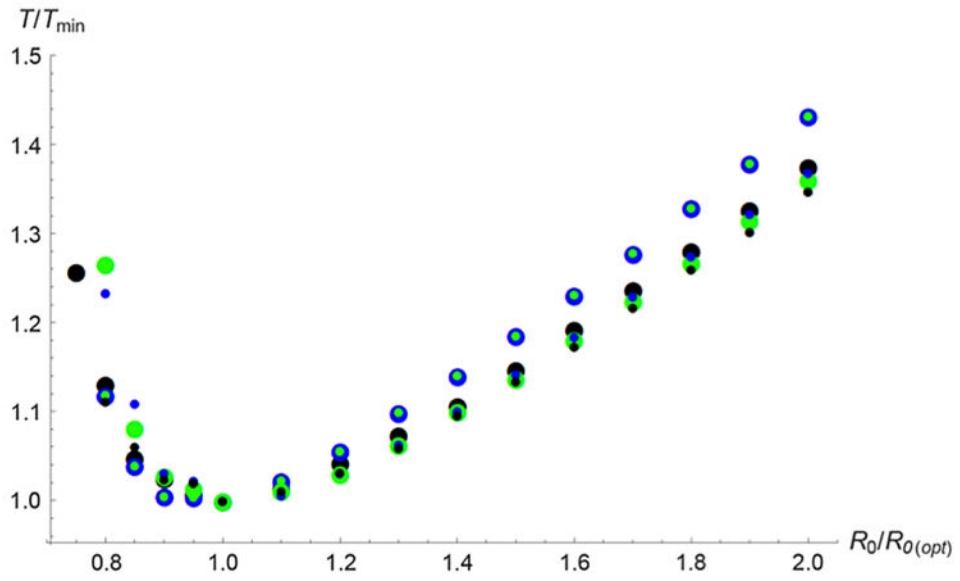
Fig. 8. Time to reach about 80% ( \sim \pi/4 ) coverage, relative to the minimum time, as a function of release area. For each model, release areas are measured relative to the release area, R_{I(opt)} , that produces T_{\min} for that model. The DTDS calculations assume Caspari-Watson dynamics with \rho = 0.2 and p_0 = 0.8 (i.e., releases produce an initial frequency of 0.8 over 20% of the target area). The small dots are produced with \hat{p} = 0.2 ; the large dots with \hat{p} = 0.3 . Green points are for Gaussian dispersal, blue points for Laplace, and black for ExpSqrt.
