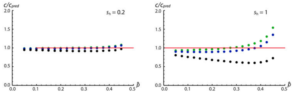
Fig. 3. Wave speed. Speed calculated from DSDT analyses compared to the cubic-based diffusion prediction, c = \sigma \sqrt{s_h} (1/2 - \hat{p}) , as a function of \hat{p} , for s_h = 0.2 (left) and s_h = 1 (right). As in (2), \sigma denotes the standard deviation of dispersal distances; s_h denotes the intensity of CI. The green dots were produced with Gaussian dispersal, blue with Laplace and black with Exponential Square root (ExpSqrt).
