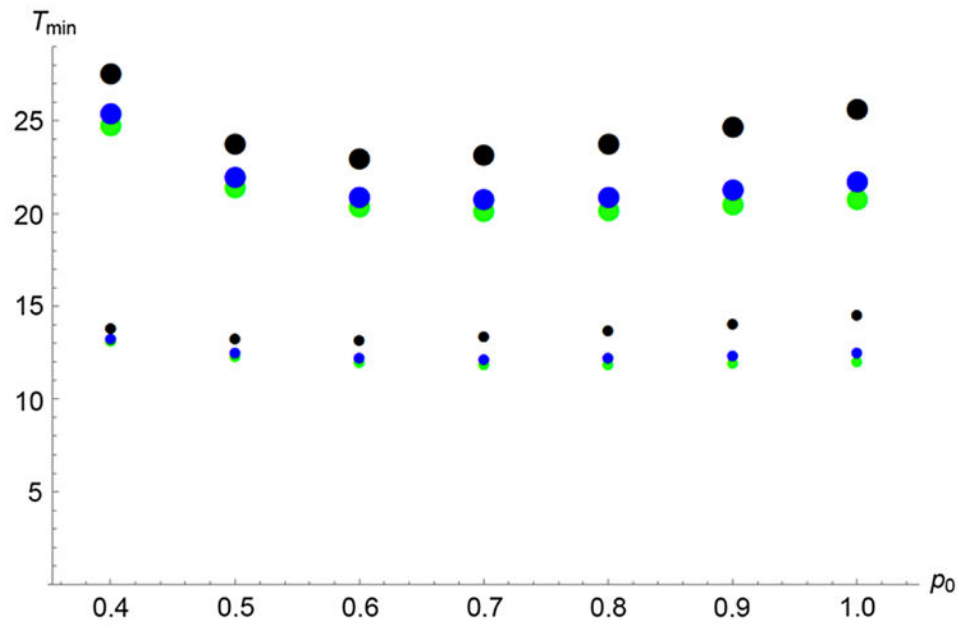
Fig. 7. Time to reach about 80% ( \sim\pi/4 ) coverage as a function of initial frequency in the release area, \rho_0 . The calculations assume \rho p_0 = 0.2 , where \rho is the fraction of the target area over which releases occur. The small dots are produced with \hat{p} = 0.2 ; the large dots with \hat{p} = 0.3 . Green points are for Gaussian dispersal, blue points for Laplace, and black for ExpSqrt.
