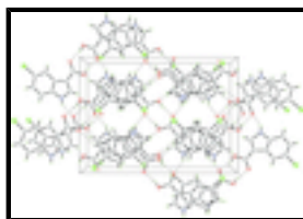
Fig. 2. A packing view down the a axis showing hydrogen bonds as dashed lines.
