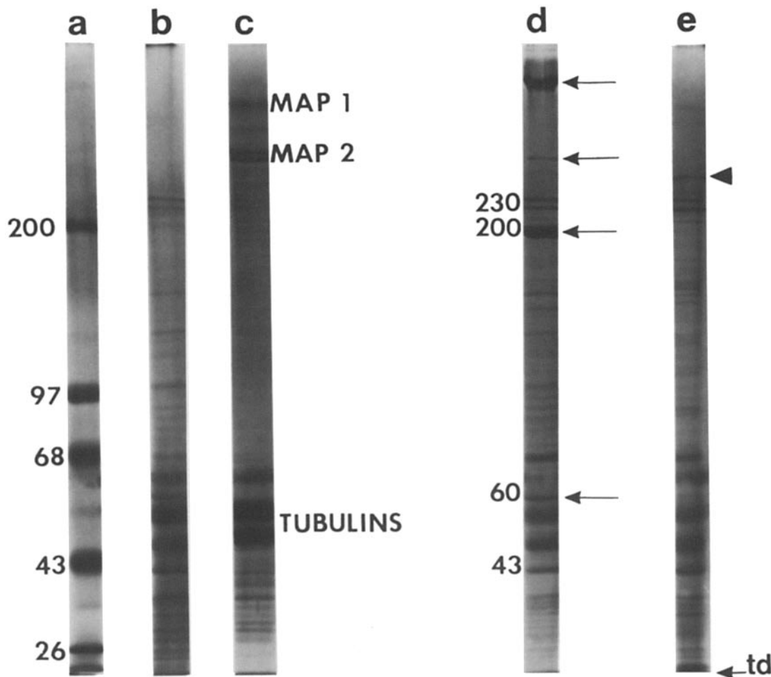
FIGURE 4 SDS PAGE analysis of the protein composition of axoplasm and of isolated vesicles. All lanes are from the same slab gel and are stained with Kodavue. Lanes a, b, and c represent standard lanes: (lane a) containing molecular weight markers ( \times 10^{-3} ); (lane b) whole axoplasm; and (lane c) purified mammalian brain microtubules. Lane d demonstrates the polypeptide composition of the vesicle pellet before the trypsin treatment. The arrows in lane d indicate the four main bands that were lost after trypsin treatment. The arrowhead (lane e) indicates a fragment of M_r 256,000 generated by the tryptic digestion. td, tracking dye.
