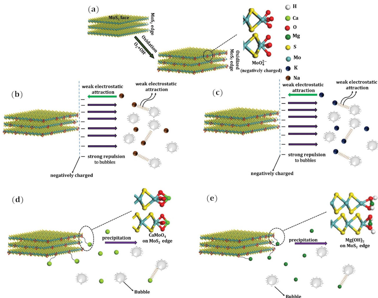
Fig. 7 Schematic of molybdenite oxidation and flotation in the presence of various cations. (a) Oxidised molybdenite edge, in the presence of (b) Na + , (c) K + , (d) Ca 2+ , and (e) Mg 2+ .
