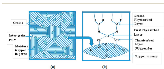
Fig. 7 (a) The inter-grain pore structure of the ZnO nanoparticles containing water vapor and (b) chemical and physical adsorption of water molecule layers on a grain along with oxygen vacancies.
