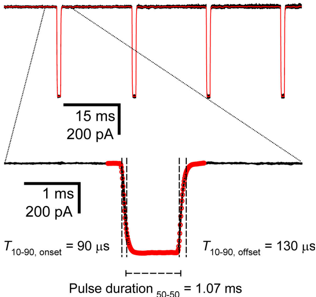
Figure 4. Calibration of the solution-switching system. The different parameters of the solution-switching system (i.e., diameter of the theta tube openings, relative positioning of the theta tube and patch pipette, flow rate of solutions, bandwidth of the computer-generated waveform) were adjusted so as to optimize the time course of the solution exchange. The latter was estimated by measuring the liquid junction potential by alternatively exposing the tip of an open pipette to 1 M KCl (for \sim 1 ms) and 140 mM KCl (for \sim 20 ms) solutions. In this particular recording, 48 1-M pulses were applied. The trace was segmented in 12 groups of four pulses, and these were aligned and averaged (red trace). The 10–90% risetime during both the onset and the offset, as well as the duration of exposure to the 1 M KCl solution, are indicated for this representative recording.
