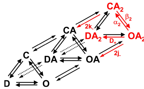
Figure 1. An allosteric reaction mechanism for the muscle AChR. C, O, and D denote the closed, open, and desensitized conformations of the channel, whereas A denotes a molecule of ACh. For simplicity, only one of the (probably several) desensitized conformations is included in the model. Also, the two neurotransmitter binding sites are assumed to be functionally equivalent and independent and, therefore, the two possible monoliganded configurations are considered to be functionally indistinguishable. These simplifications have no consequences on the interpretation of our data. The red arrows indicate the rate constants that, according to Eq. 1, determine the kinetics of the macroscopic current decay upon stepping the concentration of ACh from saturating to zero (i.e., during channel deactivation).
