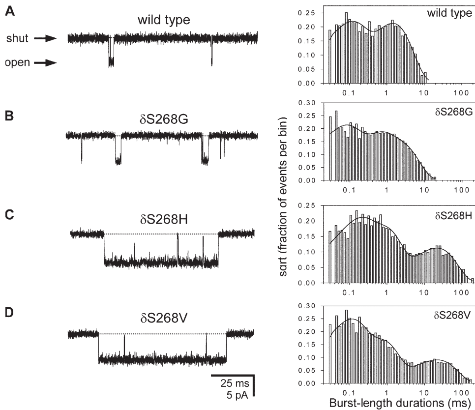
Figure 3. Burst length distributions. Example bursts of single-channel openings, and burst length duration histograms corresponding to recordings obtained from individual patches. Currents were recorded at -80 mV in the steady presence of 100 nM ACh. Openings are downward deflections. Display f_c \cong 6 kHz. The zero-current level is indicated, on each trace, with a dotted line. Bursts were defined using the criterion of Jackson et al. (1983) as outlined in Materials and methods. The time constant of the slowest component of the burst length distribution, the t_{crit} value, the total number of analyzed events (i.e., openings plus shuttings), and the fraction of misclassified shuttings in the particular cases shown are, respectively: (A) 1.29 ms, 0.27 ms, 5,691 , 0.0022 ; (B) 1.76 ms, 0.22 ms, 25,505 , 0.054 ; (C) 19.5 ms, 1.48 ms, 11,493 , 0.047 ; (D) 19.6 ms, 0.85 ms, 10,183 , 0.028 . The plotted bursts, especially in the cases of the His and Val mutants, are among the longest bursts in their respective distributions. The “length” of a burst includes the durations of all openings and shuttings within it.
