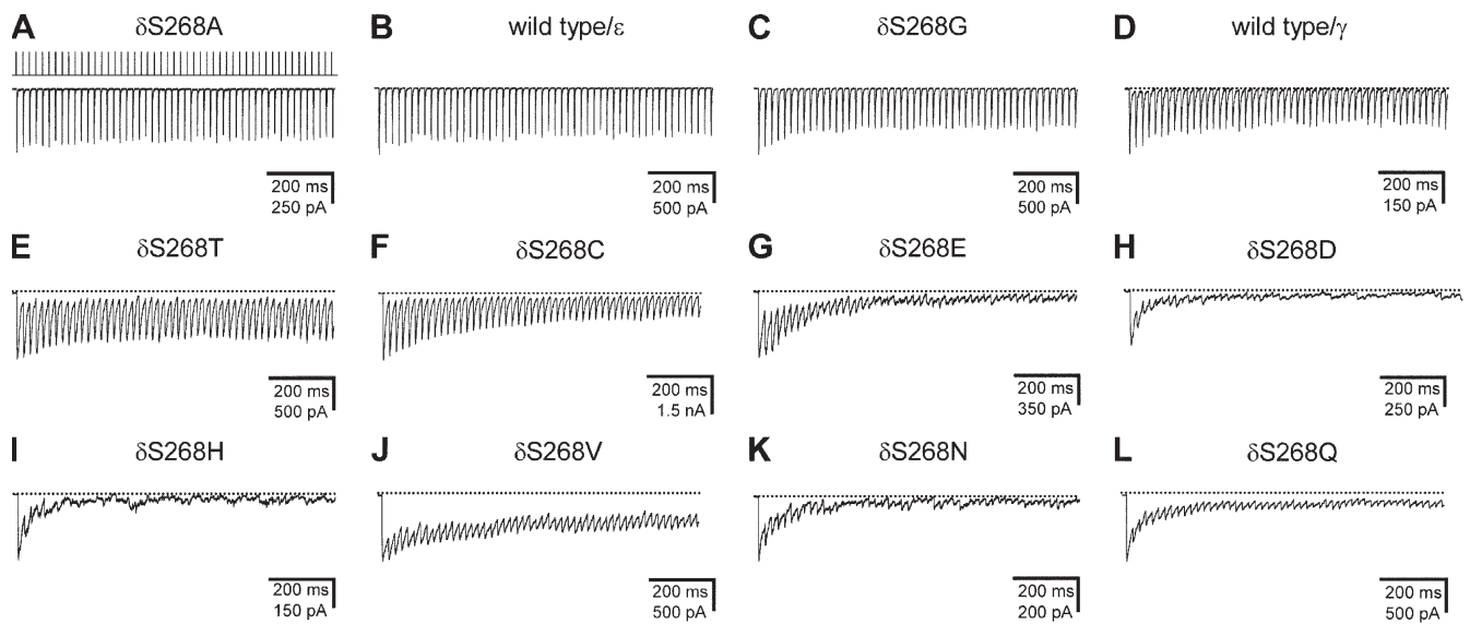
Figure 5. Gain-of-function AChR mutants desensitize during deactivation. The hypothesis that mutant AChRs desensitize upon neurotransmitter removal was tested in the outside-out configuration with the application of high-frequency trains of brief ACh pulses. (A–L) Example current traces from individual patches. Each panel is the response of a different construct to the application of a 50-Hz train of 1-ms, 100 \mu M ACh pulses. One such train is indicated in A above the current trace. The zero-current level is indicated, on each trace, with a dotted line. The plots are presented in increasing order of deactivation time constant (Table I). The prediction of Eq. 2, namely that (everything else being equal) the slower the deactivation time course, the more pronounced the depression, is borne out by these recordings. Of course, because the kinetics of entry into and recovery from desensitization are not completely unaffected by the mutations (i.e., “everything else” is not exactly equal; Table I), this relationship cannot be perfect. However, the trend is, undoubtedly, clear (see also Fig. 6).
