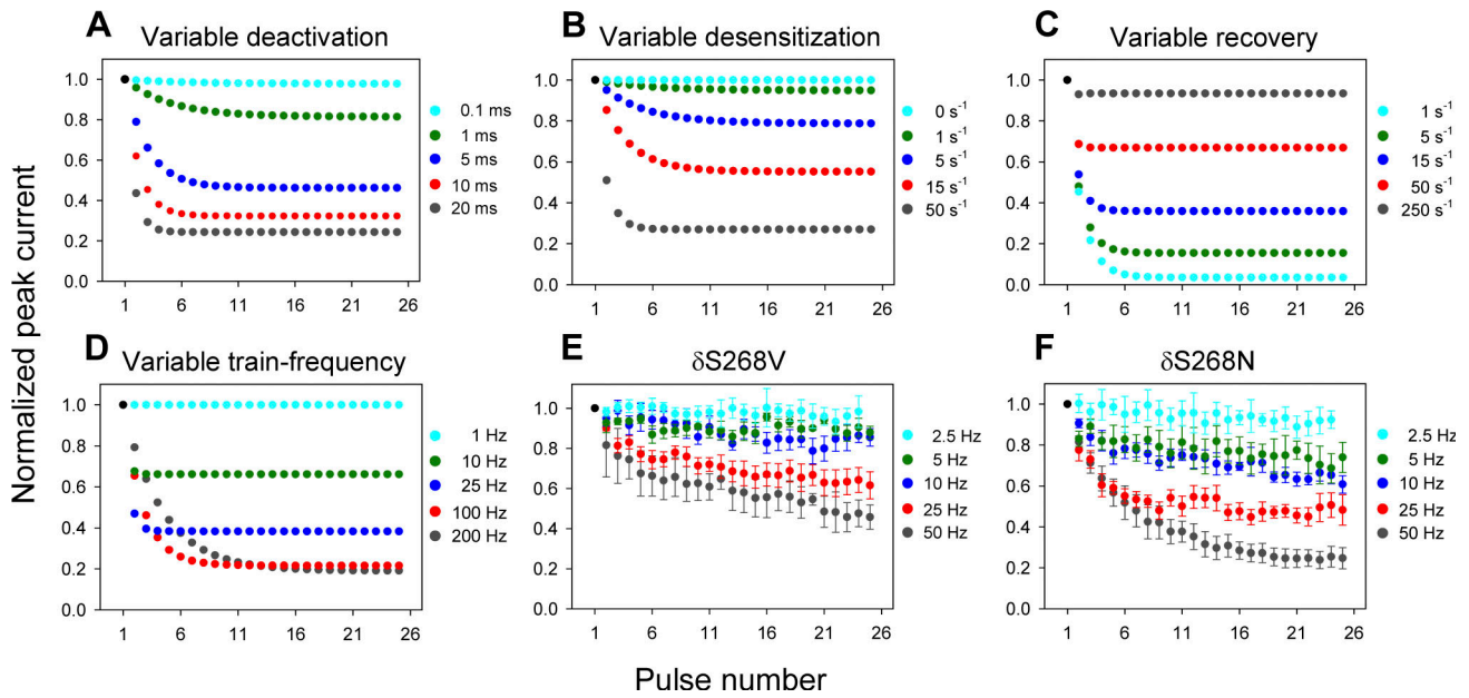
Figure 10. Effect of different variables on the macroscopic response to trains of brief neurotransmitter pulses. (A–D) Normalized peak current values under different hypothetical situations. These plots were generated by analytically solving for the fraction of channels that become activated upon each successive pulse, using the kinetic scheme in Fig. 9 A. Although these calculations do not distinguish between activated closed ( CA_2 ) and activated open ( OA_2 ) receptors, the fraction of activated channels that are open is expected to be large in the case of wild-type and gain-of-function mutant AChRs ( \sim 0.95 in the case of the adult wild-type receptor). Thus, the calculated fraction of activated channels is a good approximation to the fraction of open channels. Unless otherwise indicated, \tau_{\text{deactivation}} = 15 ms, desensitization rate constant = 50 \text{ s}^{-1} , recovery rate constant = 10 \text{ s}^{-1} , and train frequency = 50 \text{ Hz} . Each arriving pulse of ACh is considered to be too short for desensitization within a pulse to be appreciable, and is assumed to convert all activatable receptors into activated ones. The latter is a very good approximation because, using the full model in Fig. 1 and adult wild-type rate constant values, it can be calculated (using Q-matrix methods; Colquhoun and Hawkes, 1995) that \sim 90\% of all activatable AChRs would be activated by the end of a 1-ms, 100 \mu\text{M} ACh pulse. (E and F) Experimental data from two of the gain-of-function mutants exposed to trains of different frequencies. Vertical error bars are standard errors. The y axis value corresponding to the first pulse in each train (black circles) is the same for all trains.
