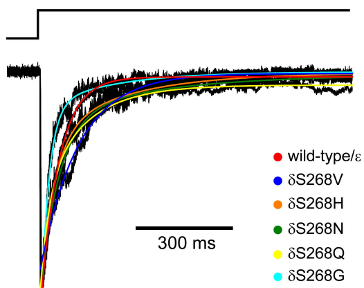
Figure 7. AChR desensitization. The kinetics of entry into desensitization were estimated by exposing outside-out patches ( -80 mV) to 2-s, 100 \mu\text{M} ACh pulses. As shown by the example current traces, opening is a transient event. For clarity, only the responses of some of the studied constructs are shown. All traces were aligned and normalized, and their decaying phases were fitted (least-squares method) from the peak of the currents until the end of the 2-s ACh applications with one or two exponential components (only the first second is shown). The parameters of these fits were used to calculate desensitization half-times (see Materials and methods). The corresponding averages, over a number of responses per construct, are listed in Table I.
