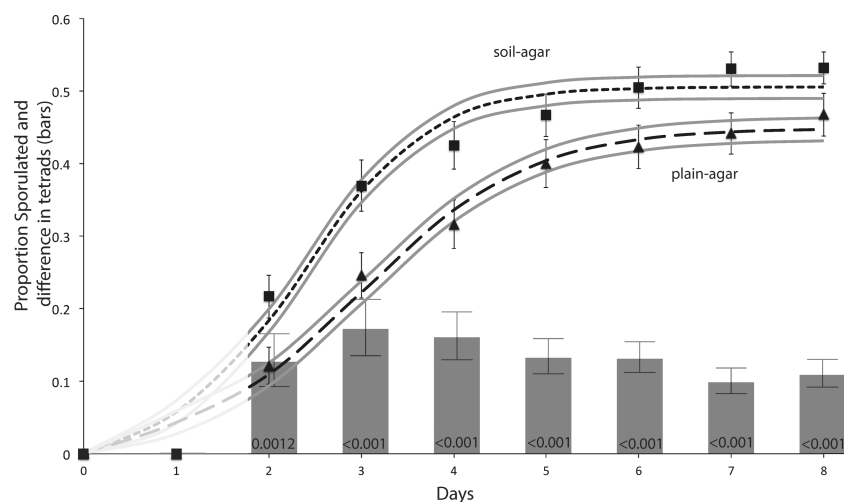
Figure 3. Sporulation dynamics across eight days, showing the mean ( \pm s.e.) in plain-agar (triangles) and soil-agar (squares) environments. The best-fit three-parameter asymptotic exponential model is shown for both: soil-agar = small dash; and plain-agar = long dash. The standard error for each curve is shown as light grey lines. The model is greyed out prior to 2 days as no sporulation was recorded. The histogram is at the same scale as the rest of the plot and shows the mean ( \pm s.e.) difference in the proportion of tetrads between the two environments at each time point: the positive values show greater tetrad number of in the soil-agar environment. The probability values for t-tests evaluating whether the difference in tetrad proportions are different from zero (i.e. that tetrad proportions do not differ between plain- and soil-agar environments) are shown at the bottom of each bar and have been adjusted for multiple comparisons using the Benjamini–Hochberg method (Benjamini and Hochberg 1995).
