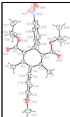
Fig. 1. ORTEP view of the molecule with the displacement ellipsoids drawn at the 40% probability level. H atoms are shown as small spheres of arbitrary radii.
