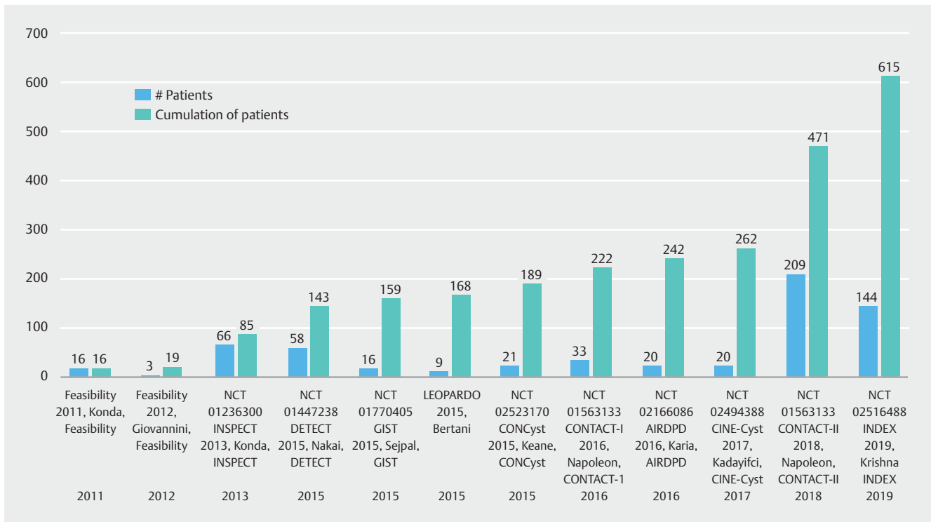
► Fig. 1 Cumulative number of patients enrolled in clinical trials evaluating EUS-guided needle based confocal laser endomicroscopy of pancreatic cystic lesions.
