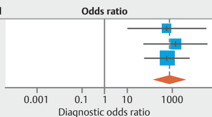
► Fig. 5 Needle-based confocal laser endomicroscopy a pooled sensitivity, b specificity, c negative predictive value, d positive predictive value, e accuracy, and f diagnostic odds ratio for mucinous lesion diagnosis. OR, odds ratio.
