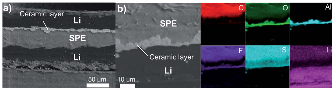
Fig. 10 SEM cross-section view and corresponding elemental mapping of an asymmetric LiAl/SPE/LiAl stack with a \sim 5 \mu\text{m} thick 50% \text{Al}_2\text{O}_3 -ndI ceramic layer on the surface of only one lithium foil. The cell assembled with this stack has been cycled at C/4 for several hundred hours and stopped before a short circuit happened. SEM cross-section views and corresponding elemental mapping for the asymmetric LiAl/SPE/LiAl stack that has been cycled at 1C for several hours (Fig. 9d) are shown in Fig. 11. The ceramic layer is still in good contact with the lithium electrode, although at some places, cracks are visible in the ceramic. However, this side is quite well conserved despite the harsh cycling at 1C. In contrast, the polymer side is strongly deformed and partially destroyed with inclusion of lithium inside the SPE (i.e. dead lithium) revealing the evident formation of dendrite during the plating process on this side. The difference is well visible in Fig. 11 with the elemental mappings of sulfur (sulfur is coming from the lithium salt used) or lithium for instance. Clearly, on the polymer side, lithium penetration into the SPE is visible. These observations are consistent with the asymmetric behavior observed at high current for the coin-cell assembled with this stack (see Fig. 9d).
