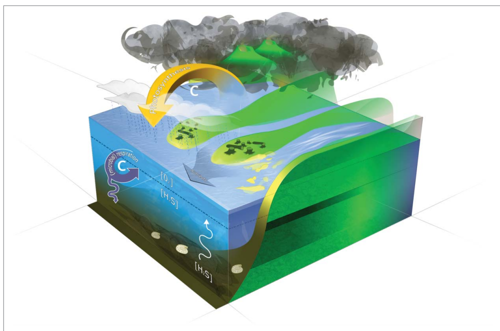
Figure 1. A conceptual model for the productivity feedback as envisioned for the latest Permian. In the sketched scenario \text{CO}_2 -outgassing associated with emplacement of the Siberian Trap basalt is held responsible for climate warming and consequential increased continental weathering by an amplified hydrological cycle but also massive destruction of vegetation. Increased river discharge (here depicted as a braided river system) supplies the ocean with excess nutrients. Eutrophication of the ocean starts a vigorous carbon loop within the water column where, among other metabolic pathways, microbial-sulfate reduction plays a pivotal role. Artwork by Mark Schobben.
