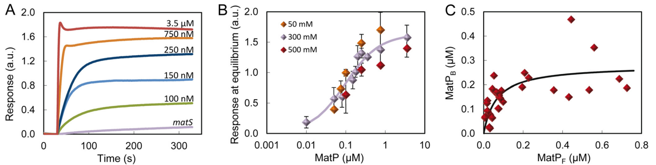
FIG 3 Binding of MatP to E. coli lipids by bilayer interferometry or using lipid-coated microbeads. (A) Representative profiles of the binding of MatP at the indicated concentrations obtained by bilayer interferometry. The profile for matS is shown for comparison. (B) Dose-response curves obtained as a function of the concentration of MatP in working buffer with the indicated KCl concentrations. The solid line is the best fit of the model explained in the main text to the data at 300 mM KCl, rendering the following parameter values: c_{50} = 0.097 \mu\text{M} and y_{\text{max}} = 1.6 . (C) MatP binding to E. coli lipid-coated microbeads in working buffer plotted as a function of the concentration of free MatP. Symbols represent the data, and the solid line represents the best fit according to the model explained in the main text rendering the parameter values c_{50} = 0.065 \mu\text{M} and y_{\text{max}} = 0.280 \mu\text{M} . The concentration of the beads is 35 g/liter (62 \mu\text{M} accessible lipid). MatP was labeled with Alexa 488.
