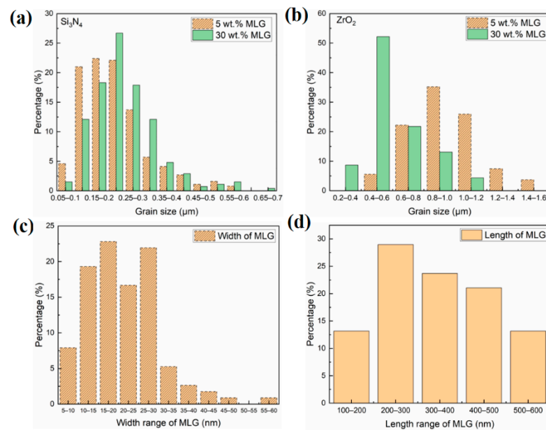
Figure 4. Histograms of size distribution for \text{Si}_3\text{N}_4 (a), \text{ZrO}_2 (b), and MLG (c,d) in the sintered composites with different graphene content, analyzed from SEM and TEM images.
