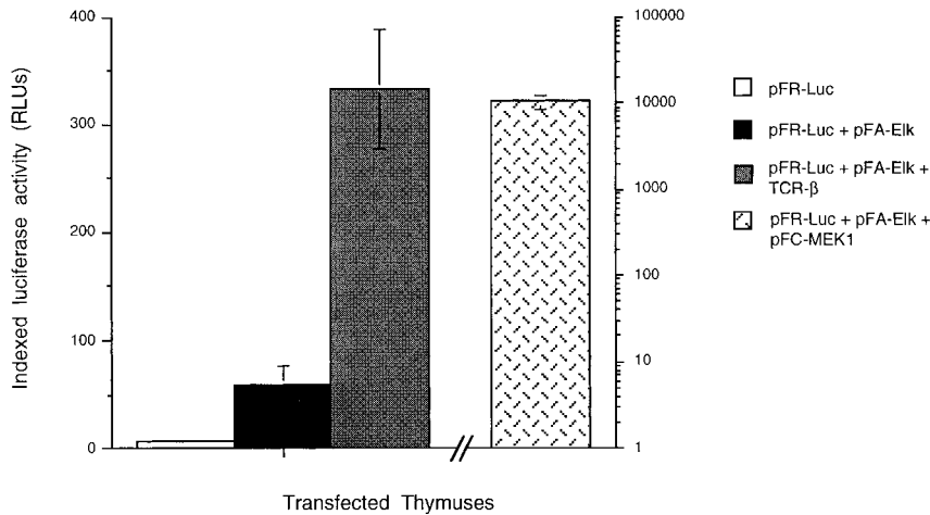
Figure 4. Activation of the ERK signaling cascade in fetal thymic lobes gene gun transfected with a plasmid encoding a functional TCR \beta chain. Intact fetal thymic lobes removed from timed-pregnant RAG -/- mice (day 14 of gestation) were used as targets for DNA-covered gold particles as described in Materials and Methods. Fetal thymi were gene gun transfected with pFR-Luc (DLR, 250 ng) and CMV- \beta -gal (DLR, 250 ng) and either pFA-Elk (DLR, 250 ng) alone or together with TCR- \beta (DLR, 250 ng) or constitutively active MEK-1 (DLR, 250 ng), as indicated. The transfected lobes were then cultured for 16–20 h. Cells were then lysed, and the lysates were assayed for luciferase and \beta -galactosidase activity. The data shown is an average of at least five independent experiments. The individual luciferase activities were indexed against a constant \beta -galactosidase activity.
