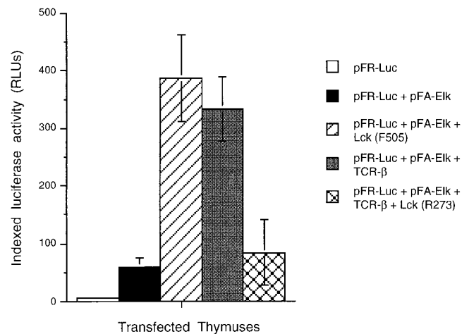
Figure 5. Activation of ERK signaling cascade by the pre-TCR is dependent on Lck function. Intact fetal thymic lobes removed from timed-pregnant RAG -/- mice (day 14 of gestation) were used as targets for DNA-covered gold particles as described in Materials and Methods. Fetal thymi were gene gun transfected with pFR-Luc (DLR, 250 ng) and CMV- \beta -gal (DLR, 250 ng) and either pFA-Elk (DLR, 250 ng) alone or together with constitutively active Lck (Lck[F505]; DLR, 750 ng), TCR- \beta (DLR, 250 ng), or TCR- \beta (DLR, 250 ng) plus dominant negative Lck (Lck[R273]; DLR, 750 ng), as indicated. The transfected lobes were then cultured for 20–24 h. Cells were then lysed, and the lysates were assayed for luciferase and \beta -galactosidase activity. The data shown is an average of at least four independent experiments. The individual luciferase activities were indexed against a constant \beta -galactosidase activity.
