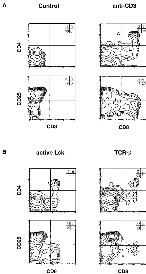
Figure 3. Generation of CD4 + CD8 + DP cells in RAG-2 -/- FTOCs gene gun transfected with plasmid encoding a constitutively active Lck or a functional TCR β chain. Intact fetal thymic lobes removed from timed-pregnant RAG-2 -/- mice (day 14 of gestation) were used as targets for DNA-covered gold particles as described in Materials and Methods. Fetal thymi were gene gun transfected with (A) control DNA and incubated in the absence (Control) or presence (anti-CD3) of 10 μg/ml anti-CD3 mAb (145-2C11) or (B) plasmid encoding a constitutively active Lck (DLR, 750 ng) or plasmid encoding a functionally rearranged TCR β chain (DLR, 250 ng). The transfected FTOCs were cultured for 7 d. After this time, a single-cell suspension was prepared and thymocytes were analyzed for surface expression of CD25, CD8, and CD4 by flow cytometry.
