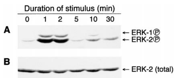
Figure 1. ERK-1/2 is phosphorylated upon cross-linking of the pre-TCR in the SL-12.12 pre-T cell line. Lysates from SL-12.12 cells stimulated with 10 \mu g/ml biotinylated anti-TCR- \beta mAb H57-597 and cross-linked with avidin (lanes 1, 2, 5, 10, and 30) or unstimulated cells (lane 0) were prepared and resolved on a 10% SDS-PAGE under reducing conditions and subsequently immunoblotted with specific antibodies against (A) phospho-ERK-1/2 and (B) ERK-2.
