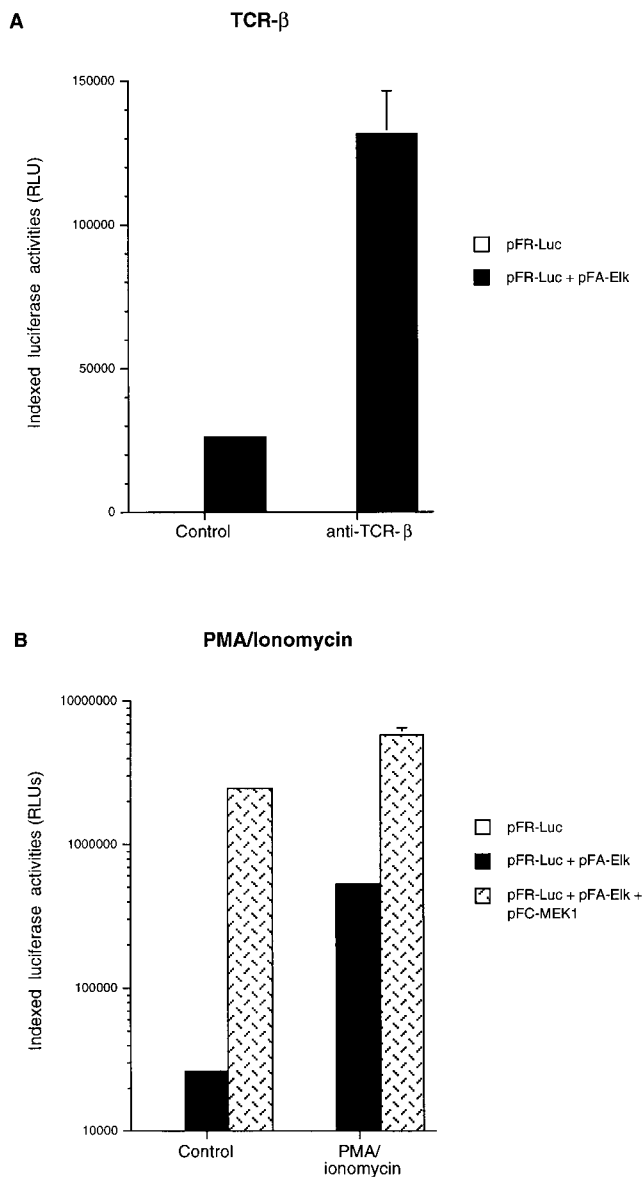
Figure 2. Activation of the ERK signaling cascade upon stimulation of SL-12 \beta .12 cells with anti-TCR- \beta mAb (H57-597; A) or PMA/ionomycin (B). SL-12 \beta .12 cells were transfected with reporter plasmids as indicated in the figure: pFR-Luc (10 \mu g), pFA-Elk (20 \mu g), and pFC-MEK1 (20 \mu g). All cells were transfected with a control \beta -galactosidase-encoding plasmid (1 \mu g). The transfected cells were incubated overnight at 37°C and then stimulated for 8 h with (A) immobilized anti-TCR- \beta or (B) phorbol ester, PMA, and the calcium ionophore, ionomycin (10 ng/ml of each). Cells were then lysed, and the lysates were assayed for luciferase and \beta -galactosidase activity. The experiment shown is representative of results carried out three times. Each experiment was carried out in triplicate, and the luciferase activities shown are indexed against \beta -galactosidase activity measured within each same sample.
