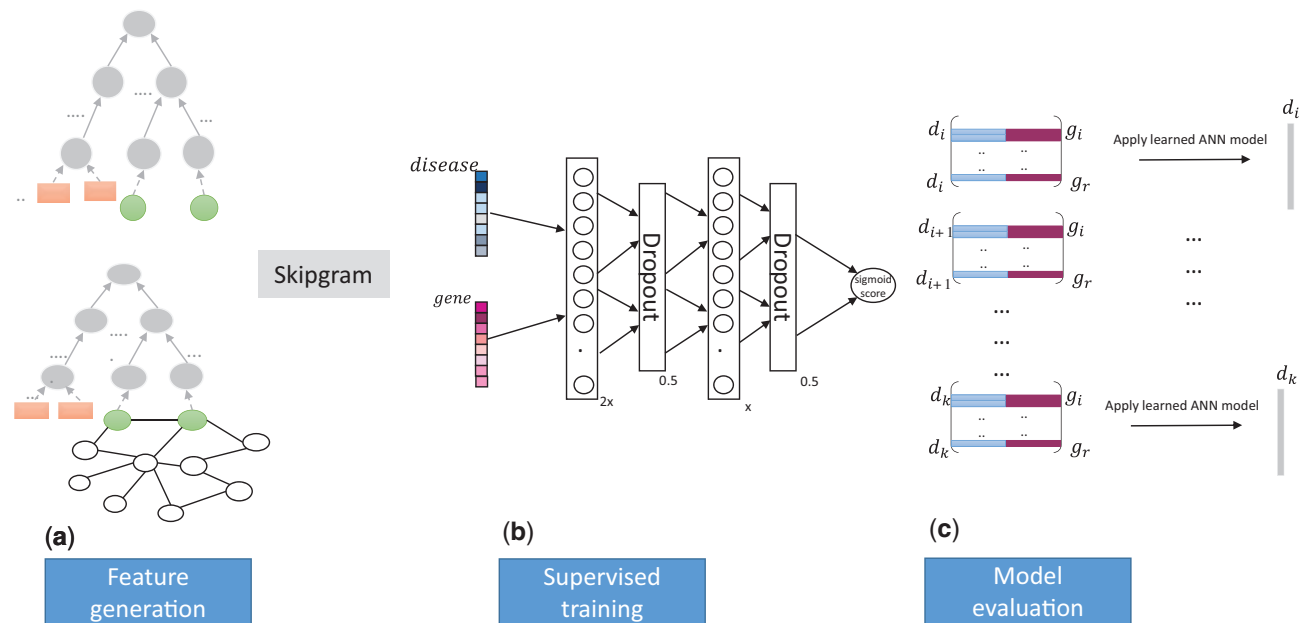
Fig. 2. Overview over SmuDGE and its applications. (a) On the left side we show the graph of disease–phenotype and gene–phenotype associations together with the PhenomeNET ontology (top), and the same graph including interactions between genes used to generate E-Vecs at the bottom. We generate a corpus by graph traversal and then use a skipgram model to generate vectors for genes and gene products in the graph. These vectors can be used as input to a similarity measure, or a neural network, to predict interactions between genes and diseases. (b) Our ANN model is shown in the center; the input is the pair of disease and gene feature vectors of dimension x , the first hidden layer consists of 2x hidden units, and the second hidden layer consists of x hidden units; we use a dropout of 0.5 to mitigate the effects of overfitting. (c) We evaluate the model by predicting candidate genes for each disease and rank each gene for each disease based on the ANN’s prediction score
