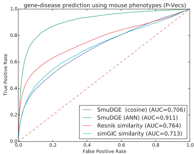
Fig. 4. Comparison of ROC curves for predicting gene–disease associations based on mouse phenotypes using SmuDGE’s feature vectors and comparison to the Resnik and simGIC semantic similarity measures
