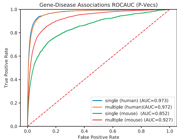
Fig. 5. ROC curves for predicting gene–disease associations for diseases with a single or multiple associated genes using SmuDGE’s P-Vec approach
