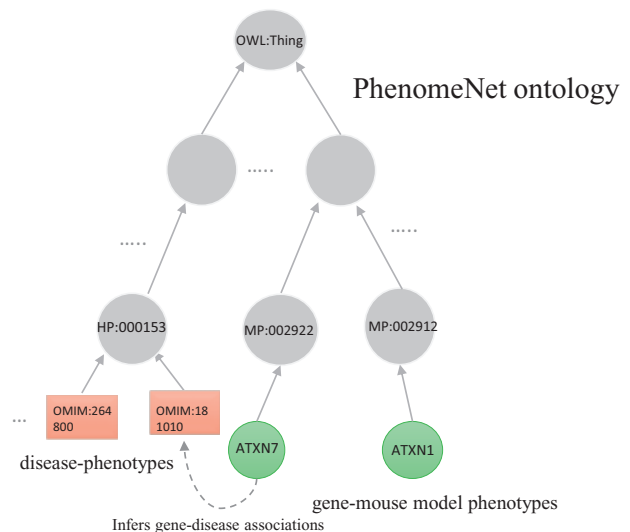
Fig. 1. Our knowledge graph consists of gene–phenotype associations (encoded using either HPO or MP), disease–phenotype associations (encoded using the HPO), interactions between genes (from the STRING database) and the PhenomeNET ontology
