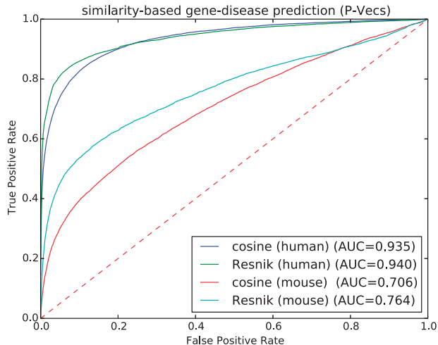
Fig. 3. ROC curves for predicting gene–disease associations using cosine similarity between SmuDGE’s P-Vecs and comparison to Resnik’s semantic similarity measure
