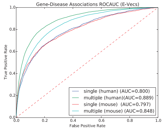
Fig. 6. ROC curves for predicting gene–disease associations for diseases with a single or multiple associated genes using SmuDGE’s E-Vec approach
