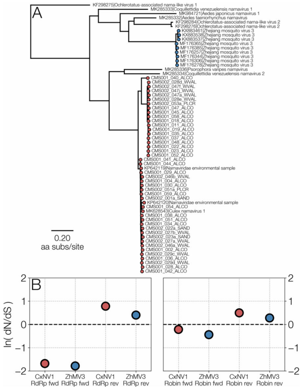
Figure 1. (A) A maximum-likelihood tree illustrating the relationship between CxNV1 ( Culex narnavirus 1) (red) and ZJMV3 ( Zhejiang mosquito virus 3) (blue) and related narnavirus RdRp amino acid sequences. (B) ORF-wide dN/dS values for forward and reverse directions of RdRp and Robin segments for both viruses.
