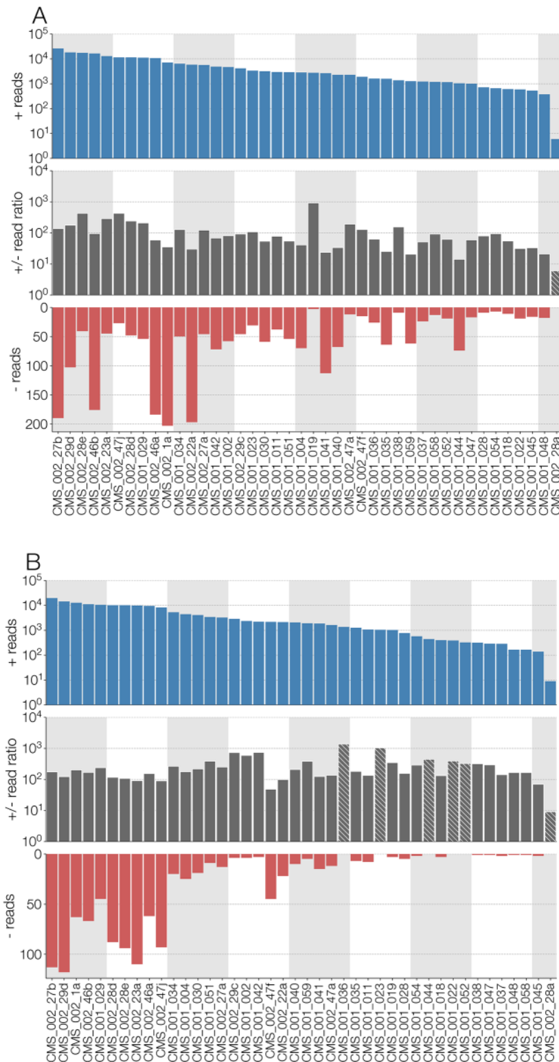
Figure 2. (A) Number of reads (from top to bottom): in the positive sense (i.e. same as genomic) with respect to RdRp segment of Culex namavirus 1 , the ratio of positive- to negative-sense reads, and negative-sense reads. Numbers of positive-sense reads and ratio of positive- to negative-sense reads are log-scaled while number of negative reads is displayed in normal space. Ratios where no negative sense reads could be identified are highlighted with hatches and the ratio reflects positive-sense reads (i.e. by assuming there is one negative-sense read). (B) Same information as A, but showing read numbers for Robin segment of Culex namavirus 1 . The results are displayed for the forty-two different strains, with the samples ordered in descending order of the total number of reads for each segment.
