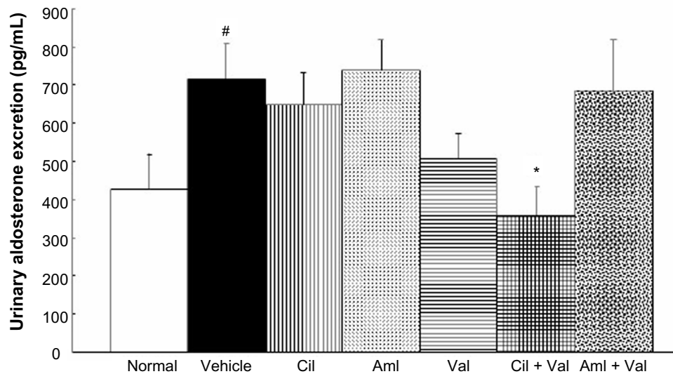
Figure 6 Effects of the combined administration of Val + Aml and Val + Cil on the levels of aldosterone. Notes: Values are means \pm standard error of the mean. # P < 0.05 versus LETO rats, * P < 0.05 versus vehicle-treated OLETF rats. Abbreviations: Cil, cilnidipine; Aml, amlodipine; Val, valsartan; LETO, Long-Evans Tokushima Otsuka; OLETF, Otsuka Long-Evans Tokushima Fatty.
