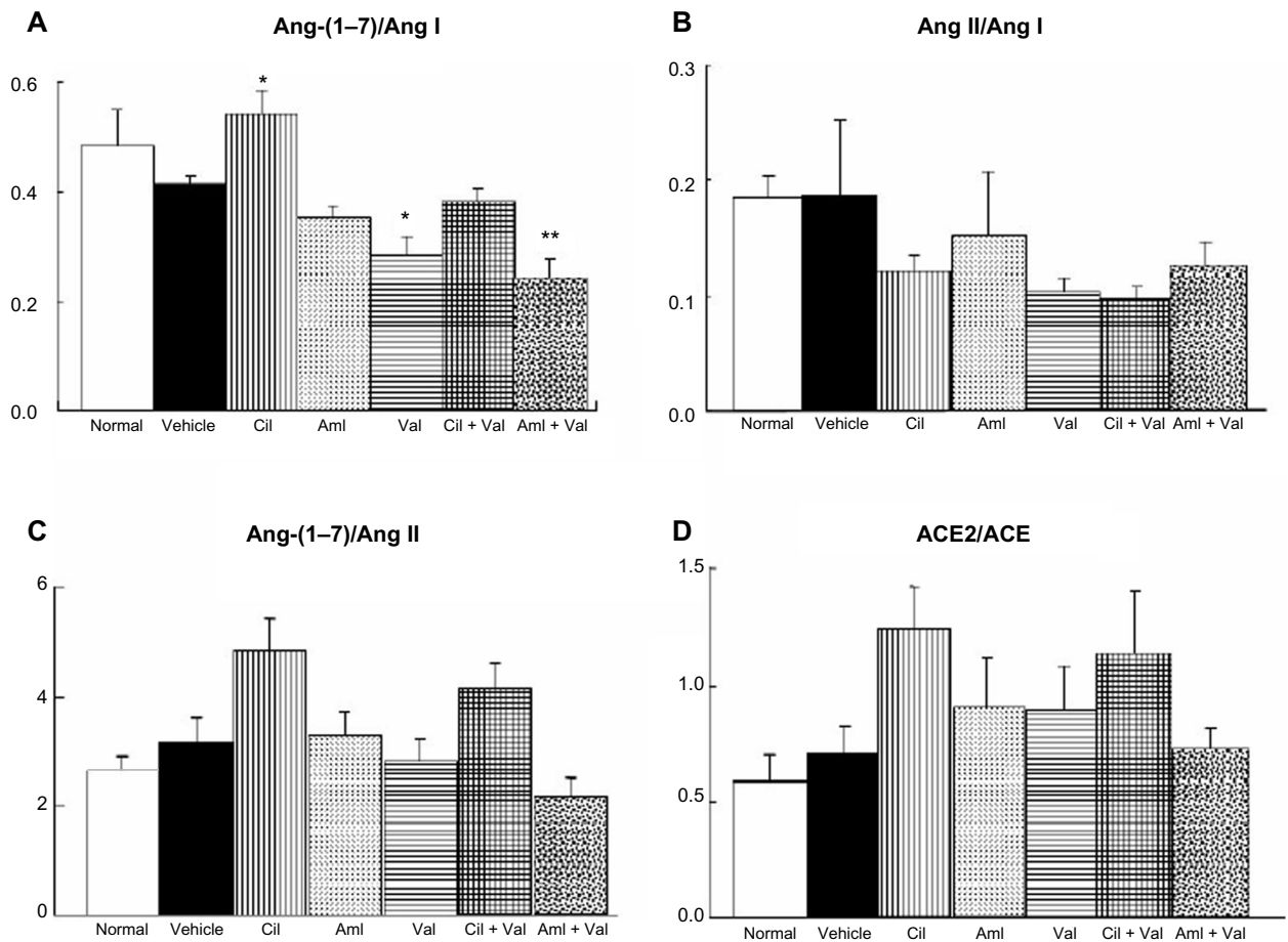
Figure 5 The ratios of angiotensin peptides and ACE2/ACE gene expression. Notes: (A) Ang-(1-7)/Ang I , (B) Ang II/Ang I , (C) Ang-(1-7)/Ang II , and (D) ACE2/ACE gene expression in the renal cortex. Values are means \pm standard error of the mean. * P < 0.05 , ** P < 0.01 versus vehicle-treated OLETF rats. Abbreviations: Ang, angiotensin; Cil, cilnidipine; Aml, amlodipine; Val, valsartan; ACE, angiotensin-converting enzyme; mRNA, messenger ribonucleic acid; OLETF, Otsuka Long-Evans Tokushima Fatty.
