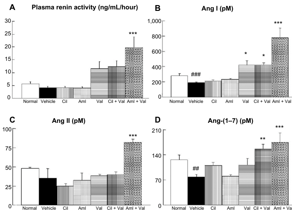
Figure 4 Effects of the combined administration of Val + Aml and Val + Cil on plasma renin activity, Ang I, Ang II, and Ang-(1-7) levels.
