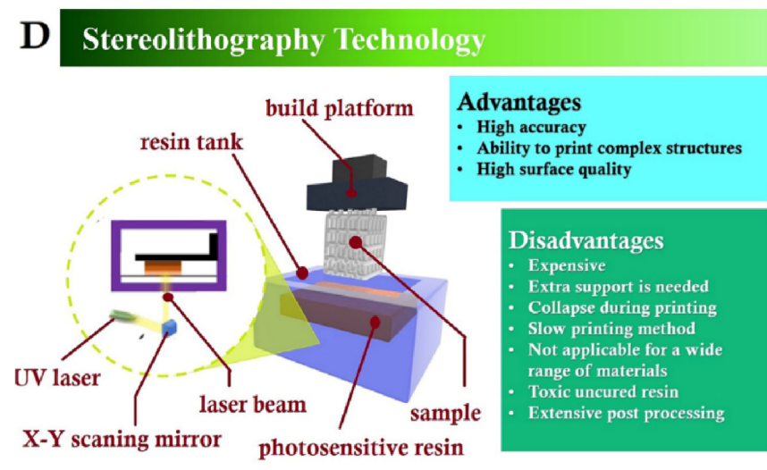
Fig. 2. Schematic representation of recognized additive manufacturing methods for printing bioceramics objects and their pros and cons, including (A) ink jetting technology, (B) selective laser sintering, (C) direct-ink writing, and (D) stereolithography.
