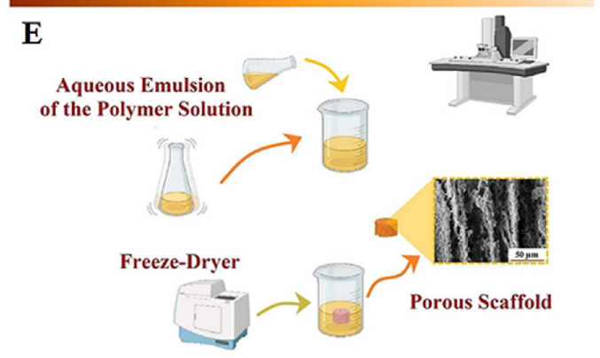
Fig. 1. (A) Baghdadite crystal structure, fabrication procedure and microstructure of (B) sintered bulk baghdadite ceramic at various sintering temperature, SEM images reproduced with permission from Ref. [38], baghdadite scaffold fabrication procedure by (C) polymer sponge method, SEM image reproduced with permission from Ref. [11], (D) space holder methods, SEM image reproduced with permission from Ref. [8], and (E) freeze-drying, SEM image reproduced with permission from Ref. [39].
