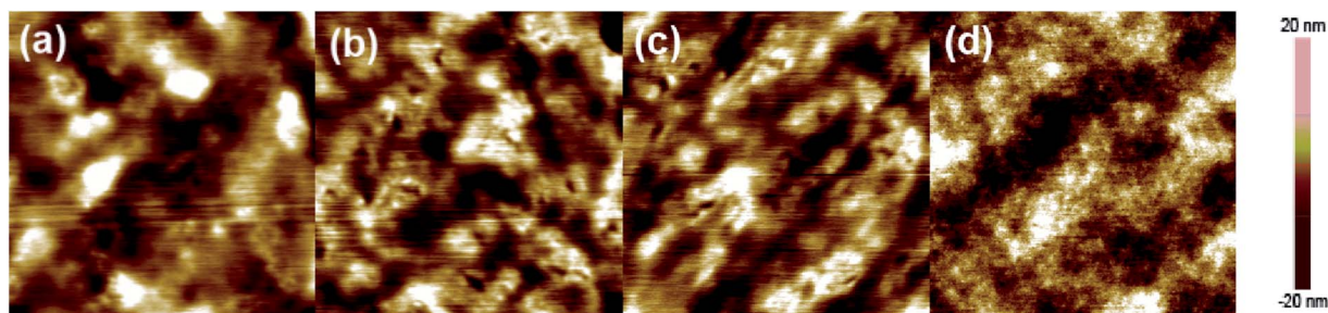
Fig. 4 AFM topography images (a–d) of J51:PC 71 BM blend thin films with J51-8kDa (a), J51-16kDa (b), J51-21kDa (c), and J51-36kDa (d) (image size: 5 × 5 μm 2 ).
