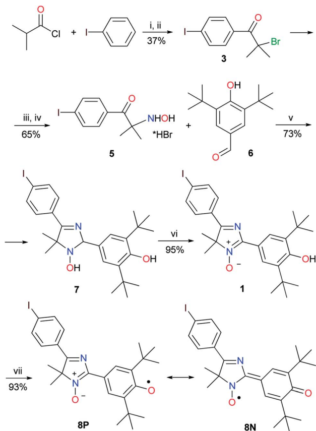
Scheme 1 Reagents and conditions: (i) \text{AlCl}_3 , 45^\circ\text{C} , 15 h; (ii) \text{Br}_2 , \text{Et}_2\text{O} /dioxane, room temperature (rt), 2 h; (iii) \text{NH}_2\text{OH} \times \text{HCl} , \text{NaOH} , \text{MeOH}/\text{H}_2\text{O} , 65^\circ\text{C} , 7 h; (iv) 48% \text{HBr} , \Delta , 2 h; (v) \text{NH}_4\text{OAc} , \text{MeOH} , rt, 6 h; (vi) \text{MnO}_2 , \text{CHCl}_3 , rt, 7 h; and (vii) \text{PbO}_2 , \text{CHCl}_3 , rt, 2 h.
