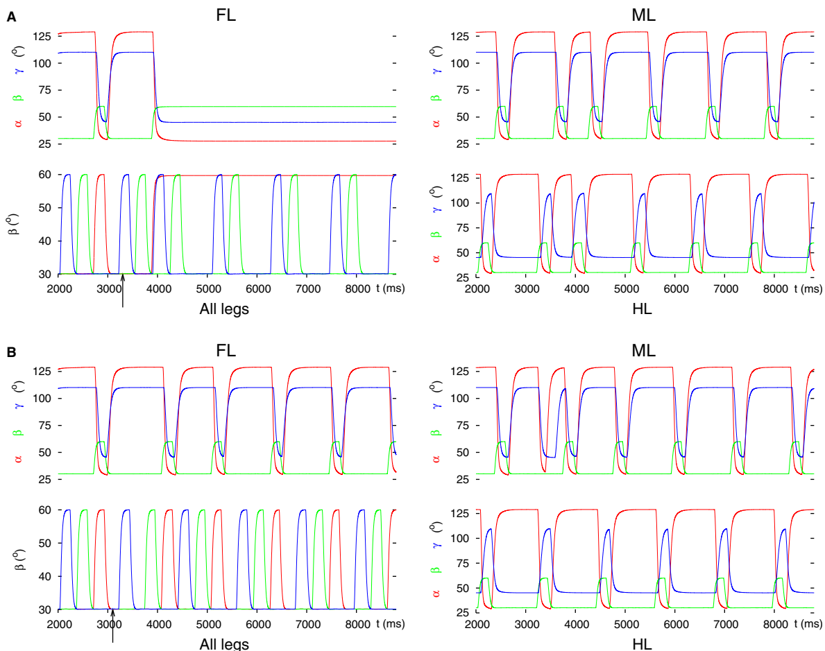
Figure 4. Successful and failed decoupling of the front leg by changing the (central) synaptic drives to the CPG of the LD system of the front leg. Depending on the phase of the stepping period at which the decoupling command is evoked, the decoupling may succeed or fail. (A) successful decoupling. Note the steady-state position of the front leg. (B) failed decoupling. The same permanent change to the drives ( g_{app3} and g_{app4} ) as in A remains ineffective. All notations are the same as in Figure 3.
