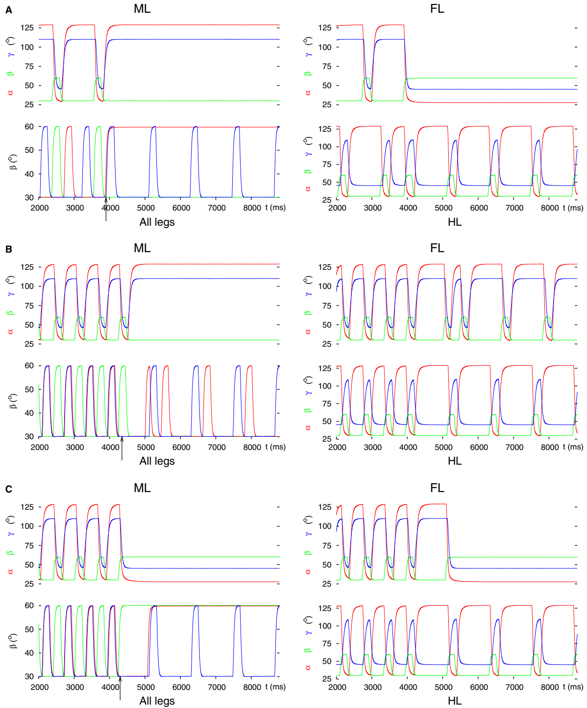
Figure 10. Decoupling of the middle leg via premotor inhibitory INs. (A) Premotor IN to the depressor MN is inhibited, while the one to the levator MN is disinhibited. As a result, the middle leg permanently remains on the ground (retracted, flexed). The front leg stays lifted (protracted and stretched), while the hind leg continues normal stepping. (B) The inputs to the premotor INs are the same as in A but the decoupling command arrives at a different phase of the stepping period. As a result, the front leg and the hind leg now perform coordinated stepping. (C) Premotor IN to the depressor MN is disinhibited, while the one to the levator MN is inhibited. The middle leg therefore stays lifted (protracted and stretched). The front leg also stays lifted as in A. Here, the starting coordination pattern in A was tetrapod, while in B and C tripod. All notations are the same as in Figure 3.
