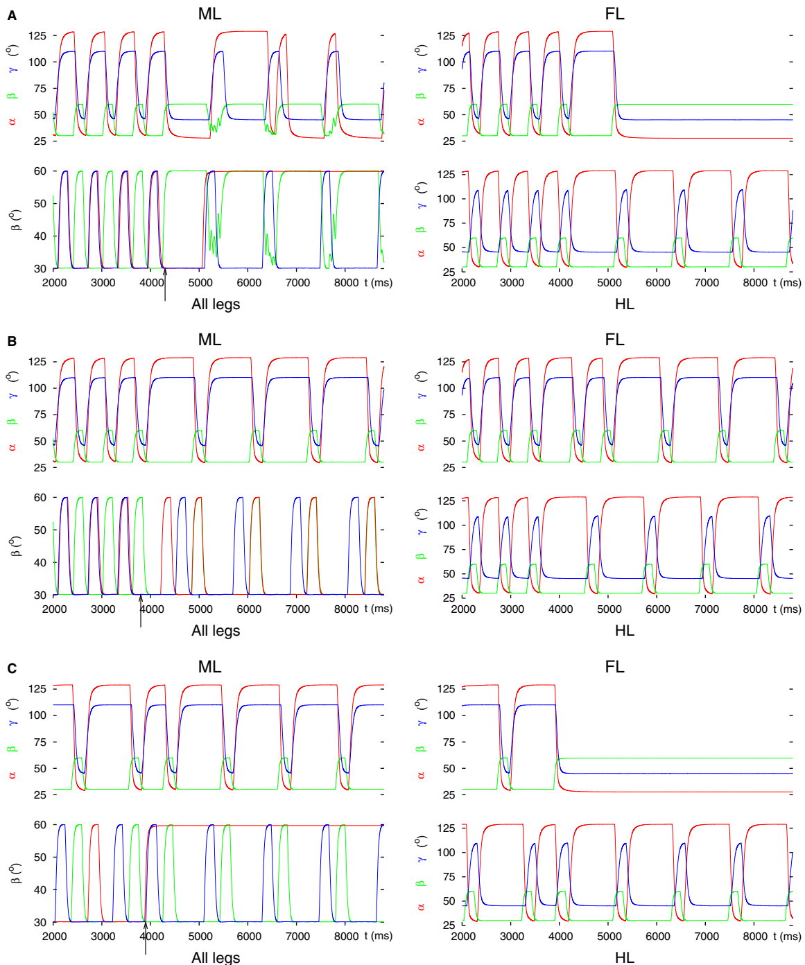
Figure 9. Decoupling of the middle leg by permanently changing the input to its LD CPG. Three typical results are illustrated. The first result was obtained by applying (strong) excitatory input to the levator and (strong) inhibitory input to the depressor CPG neuron. The second and third one arose, when there was no input to the CPG (both input conductances were set to zero; Figure 1D). (A) The middle leg does not have proper ground contact; the front leg remains lifted, protracted, and stretched; the hind leg continues its normal stepping. This result was obtained with both starting coordination patterns (tripod, tetrapod). The result displayed is with the starting coordination pattern tripod. (B) All three legs continue stepping but the front and middle leg step in synchrony. This result could only be seen with starting tripod coordination pattern. (C) The middle and the hind leg continue tetrapod stepping but the front leg remains permanently lifted (protracted and stretched). This result clearly shows a failed decoupling of the middle leg but a successful decoupling of the front leg. It occurred only with starting tetrapod coordination pattern. All notations are the same as in Figure 3.
