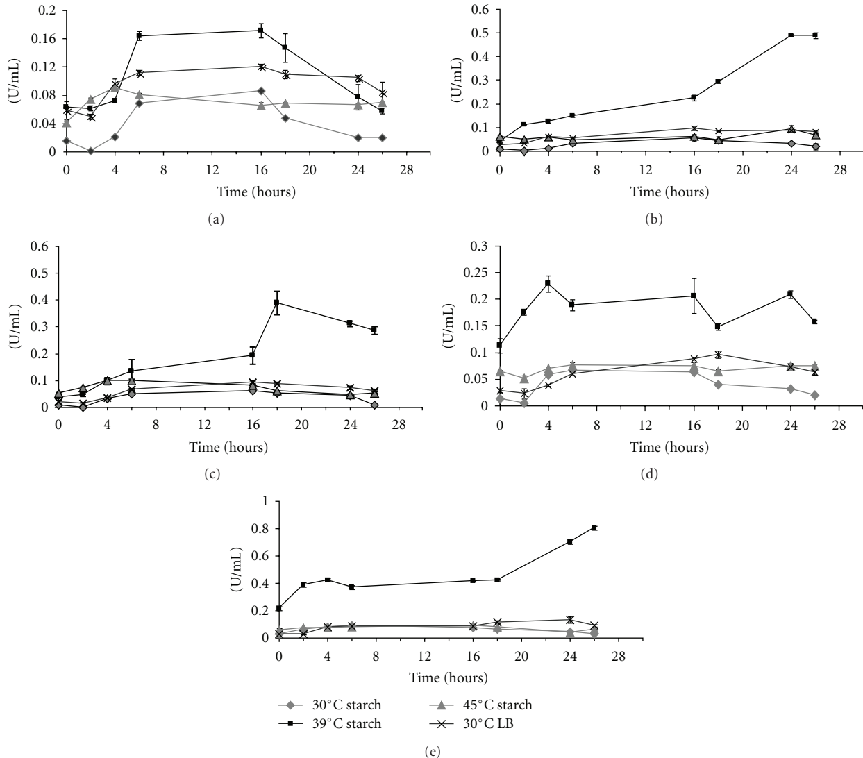
FIGURE 2: Kinetics of amylase activity in the culture supernatants of five isolates (a) URX291, (b) URX303, (c) URX350, (d) UED 641, and (e) UED644 in starch medium for 26 hours at 30 (diamonds), 39 (squares), 45°C (triangles), and in LB rich medium at 30°C (crosses). n = 9 . Vertical lines represent error bars.
