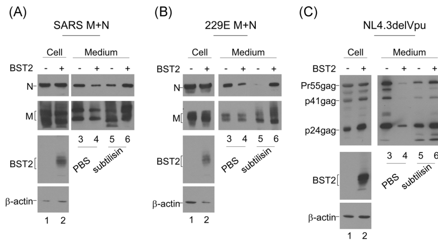
FIGURE 2 Subtilisin treatment promotes virus-like particle release. 293T cells were cotransfected with SARS CoV (A), HCoV-229E M and N (B), or NL4.3delVpu (C) with or without a BST2 expression vector. Cells were split equally into two dish plates at 24 hours posttransfection. After an additional 4 hours, culture medium was removed, washed twice with PBS, and incubated with PBS containing subtilisin (1 mg/mL) for 10 minutes at 37°C. Supernatants were harvested and centrifuged through 20% sucrose cushions, and pellets and cell lysates were subjected to western immunoblotting. Viral proteins were probed as described in the Figure 1 caption. BST2, bone marrow stromal antigen 2; PBS, phosphate-buffered saline; SARS-CoV, severe acute respiratory syndrome coronavirus
