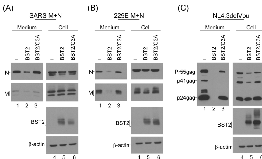
FIGURE 3 Cysteine residues in the BST2 N-terminal ectodomain are important for inhibiting VLP release. 293T cells were cotransfected with SARS M plus N (panel A), HA-tagged HCoV-229E M plus N (panel B), or NL4.3delVpu (panel C) plus a wild-type or mutant BST2 expression vector (BST2/C3A) containing alanine substitutions for three cysteine residues in the BST2 ectodomain. Cells and supernatants were harvested and subjected to western immunoblotting at 24 to 36 hours posttransfection. BST2, bone marrow stromal antigen 2; VLP, virus-like particle
