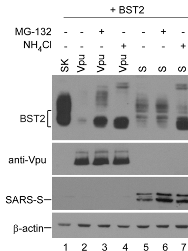
FIGURE 5 SARS-CoV S downregulates BST2 via a lysosomal degradation pathway. 293T cells were transfected with BST2 (lane 1) or cotransfected with BST2 plus a Vpu (lanes 2-4) or SARS-CoV S (lanes 5-7) expression vector. At 24 hours posttransfection, cells were either left untreated (lanes 1, 2, and 5), treated with 30 \mu M MG-132 for 6 hours (lanes 3 and 6), or treated with 25 \mu M NH 4 Cl (lanes 4 and 7) for 6 hours before harvesting and immunoblotting. BST2, bone marrow stromal antigen 2; SARS-CoV, severe acute respiratory syndrome coronavirus
