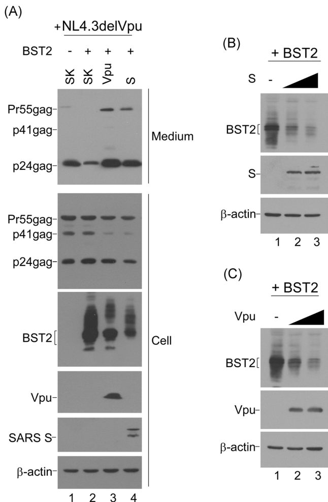
FIGURE 4 SARS-CoV S downregulates BST2. A, SARS-CoV S reduced the inhibition of HIV-1 VLP production by BST2. 293T cells were transfected with NL4.3delVpu alone (lane 1) or combined with BST2 (lane 2) plus Vpu (lane 3) or SARS-CoV S (lane 4) expression vectors. Cells and supernatants were harvested and subjected to western immunoblotting at 24 to 36 hours posttransfection. B-C, 293T cells were transfected with 100 ng of BST2 alone (lane 1) or BST2 plus 1 \mu g (lane 2) or 3 \mu g (lane 3) of a SARS-CoV S (panel B) or Vpu expression vector (panel C). Cells were harvested and subjected to western immunoblotting at 24 hours posttransfection. BST2, bone marrow stromal antigen 2; SARS-CoV, severe acute respiratory syndrome coronavirus; VLP, virus-like particle
