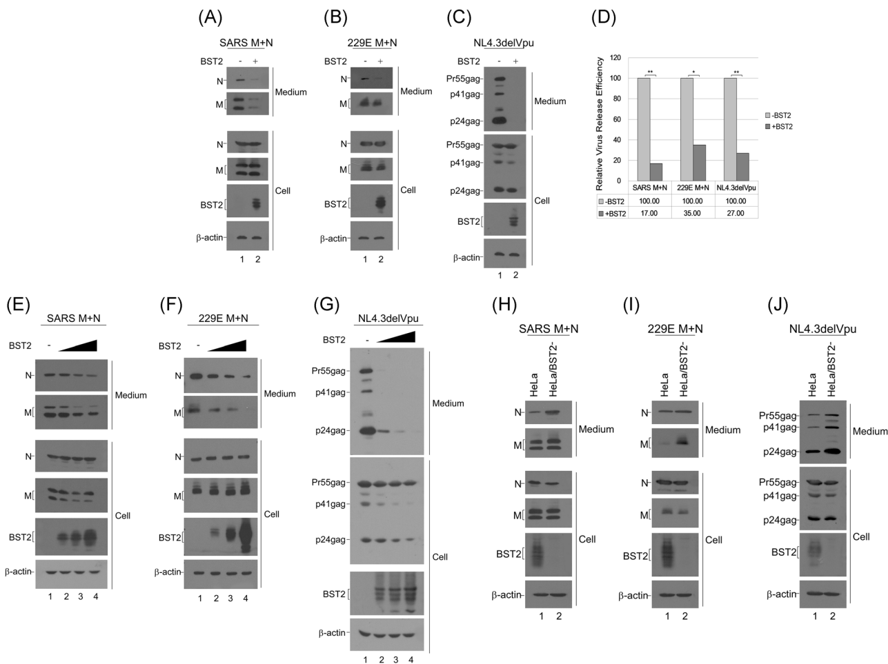
FIGURE 1 BST2 inhibits coronavirus virus-like particle (VLP) production. A-D, 293T cells were cotransfected with SARS M and N (panel A), HA-tagged HCoV-229E M and N (panel B), or NL4.3delVpu (panel C) expression vectors, with (lane 2) or without a BST2 expression vector. Cells and supernatants were harvested and subjected to Western immunoblotting at 24 to 36 hours posttransfection. D, N proteins from medium or cell samples were quantified by scanning N band densities from immunoblots. Ratios of N level in media to those in cells were determined for each sample and normalized to that of samples without BST2 coexpression. Data were derived from at least three independent experiments. * P < .05 ; ** P < .01 . (E-G) 293T cells were transfected with SARS (panel E), HCoV-229E (panel F), or HIV-1 (panel G) VLP-producing expression vectors as described for (A-C). All tests were performed with 0.1 \mu g, 0.5 \mu g, or 2 \mu g of cotransfected BST2 expression plasmids (lanes 2, 3 and 4, respectively). H-J, HeLa or BST2-knockdown HeLa (HeLa/BST2-) cells were transfected with the indicated SARS, HCoV-229E, or HIV-1 VLP-producing plasmid. Cells and supernatants were harvested, prepared and subjected to Western immunoblotting at 48 to 72 hours posttransfection. Viral proteins were detected with anti-SARS-CoV M, anti-HCoV-229 N antiserum, or monoclonal antibodies against SARS-CoV N, HA-tagged HCoV-229 M, or p24CA. BST2 was probed with a rabbit anti-BST2 antibody. BST2, bone marrow stromal antigen 2; SARS-CoV, severe acute respiratory syndrome coronavirus
