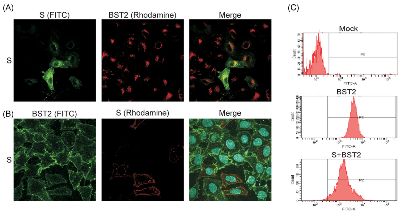
FIGURE 6 SARS-CoV glycoprotein S colocalizes with BST2. 293 cells (panel A) were cotransfected with BST2 and a SARS-CoV expression vector. HeLa cells (panel B) were transfected with the SARS-CoV S expression vector. At 24 to 36 hours posttransfection, cells were probed with an anti-BST2 antibody before cell membrane permeabilization. SARS-CoV S was probed with an anti-S polyclonal antiserum. A rhodamine-conjugated or FITC-conjugated antirabbit or antimouse antibody served as a secondary antibody. C, SARS-CoV S coexpression reduces BST2 cell surface expression. 293T cells were transfected with BST2 alone (middle panel) or together with a SARS-CoV S expression vector (bottom panel). At 24 to 36 hours posttransfection, cells were fixed and probed with a rabbit anti-BST2 antibody before the permeabilization of cell membranes, followed by a secondary FITC-conjugated antirabbit antibody. Cells then were analyzed by flow cytometry. BST2, bone marrow stromal antigen 2; SARS-CoV, severe acute respiratory syndrome coronavirus
