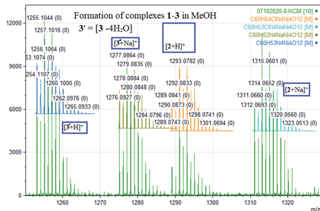
Scheme 2 Syntheses of complexes 1–3 in MeOH rationalizing the mechanism of their formation (top). ESI mass spectrometric analysis of reaction solution (bottom). S = solvent (MeOH/H 2 O).
