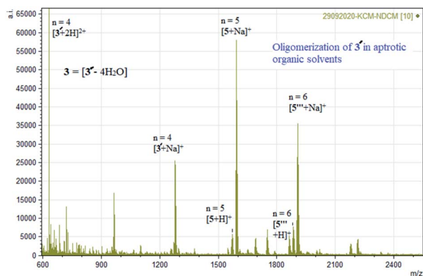
Fig. 6 Experimental mass spectrum of 3 representing oligomerization in aprotic solvent [\text{Ni}_4((\text{O}^-)_2\text{L-Me})_4] = 3' = [3 - 4\text{H}_2\text{O}] (Table 1).
