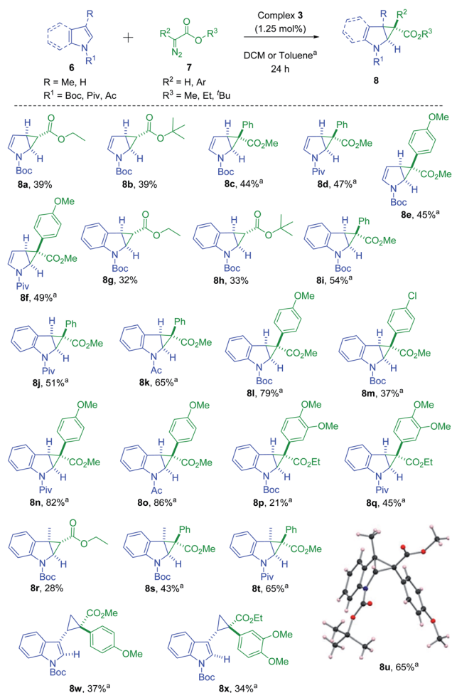
Scheme 3 Substrate scope for cyclopropanation of aromatic heterocycles catalyzed by complex 3. a The reported yields are for reactions carried out at 100 °C using an oil bath.
