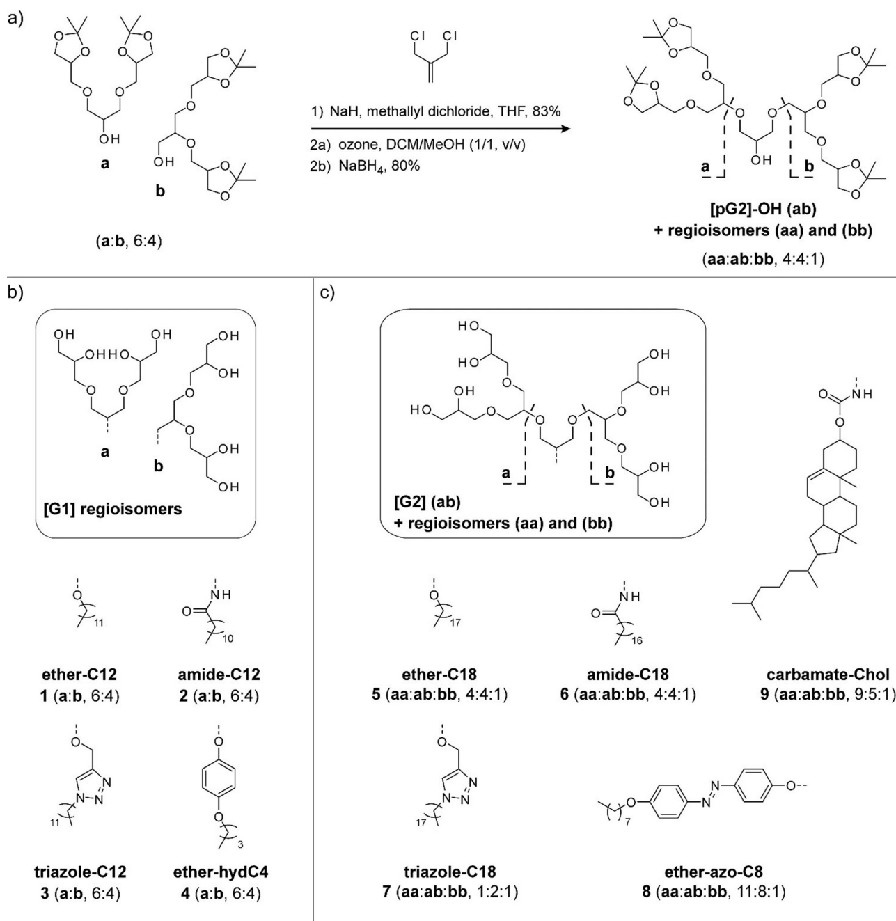
Figure 2. Synthesis of [G1] and [G2] OGD regioisomer mixtures. a) The use of a [pG1]-OH regioisomer mixture (a,b) as starting material leads to three [pG2]-OH regioisomers (aa, ab, bb), which differ in terms of the structure of their triglycerol side chains. Using [pG1]-OH and [pG2]-OH regioisomer mixtures as the starting material for detergents leads to b) [G1] and c) [G2] OGD regioisomer mixtures (for further information see the Supporting Information).
