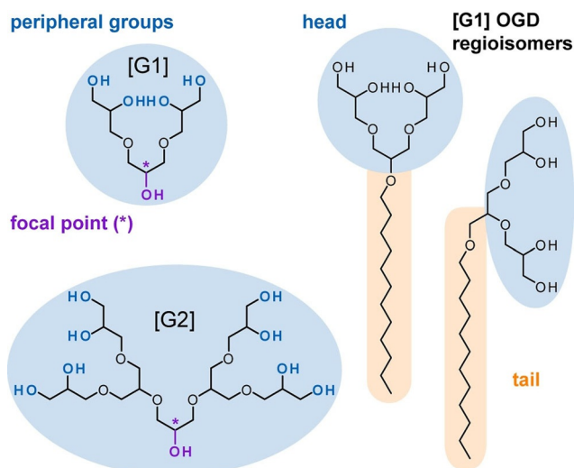
Scheme 1. First- [G1] and second-generation [G2] oligoglycerol dendrons contain a single chemically addressable functional group at the core (focal point). The number of hydroxy groups at the periphery and their size vary between the generations. Dendritic OGDs contain a hydrophilic head and a hydrophobic tail. Regioisomers differ in terms of connectivity between glycerol units in the head group. Mixtures of [G1] OGD regioisomers can extract more protein quantities from membranes than individual regioisomers. The origin of this behaviour remains elusive.
