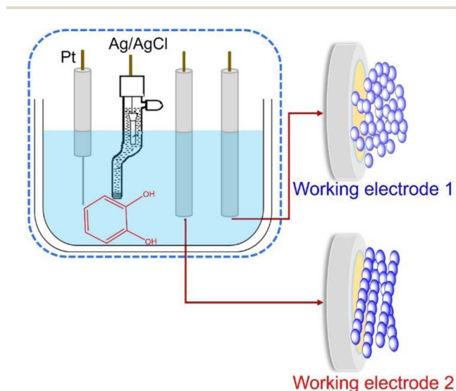
Scheme 1 Diagrammatic sketch of the dual-working electrode system.
