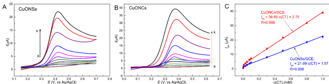
Fig. 5 LSV results for (A) CuONSS/GCE and (B) CuONCs/GCE in 0.1 M PBS (pH 7.0) containing CT at (A) (a) 0 mM, (b) 0.002 mM, (c) 0.01 mM, (d) 0.03 mM, (e) 0.05 mM, (f) 0.08 mM, (g) 0.1 mM, (h) 0.3 mM, (i) 0.5 mM, (j) 0.8 mM, (k) 1 mM. Scan rate: 50 mV s -1 . (C) Linear plots of peak current vs. concentration (4 measurements per point).
