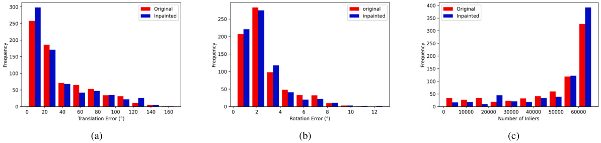
Fig. 11. Optical flow analysis: Histograms of RTE, RRE, and RANSAC Inliers for both original and inpainted sequences using Model_{T,C} .
