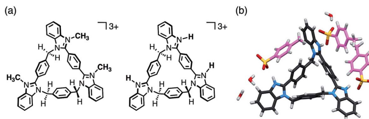
Fig. 6 (a) Chemical structures of tri-methylated and tri-protonated anti-3 . (b) Crystal structure of [\text{H}_3(\text{anti-3})(\text{p-TsO})_3] \cdot (\text{H}_2\text{O})_3 . Disordered water molecules are omitted for clarity. The carbon atoms of p -TsO are shown in pink.
