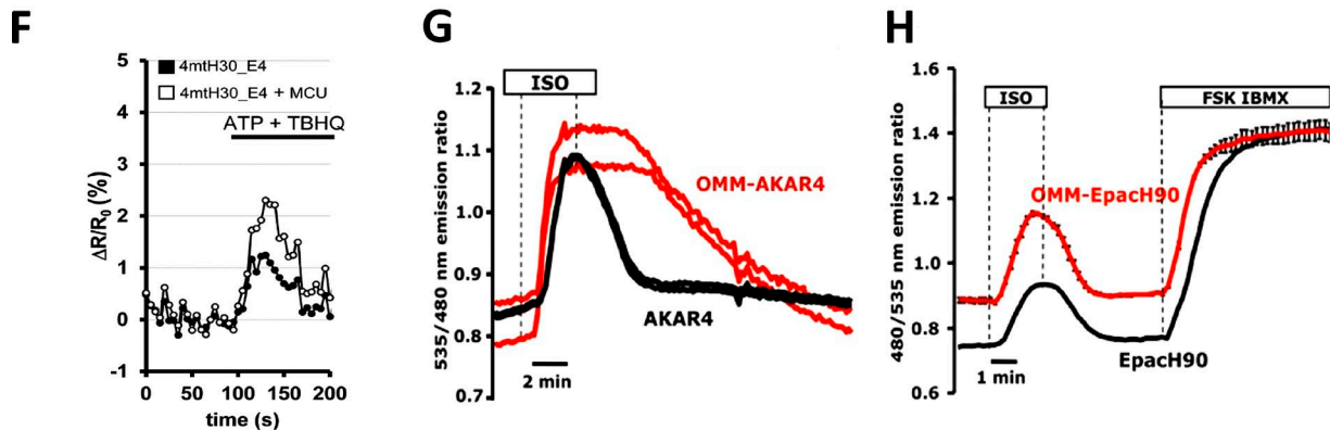
Figure 10. cAMP signaling. (A–C) Localized increases of cAMP. (A) Scanning ion conductance microscopy image and corresponding cAMP level obtained in cardiomyocytes expressing Epac1-cAMP sensor upon local \beta_2 -adrenergic receptors ( \beta_2 AR) stimulation in the cell crest (B) and in the T-tubule (C). Cells were stimulated with a \beta_2 AR agonist (ISO and CGP) in the presence of a \beta_1 AR antagonist, showing \beta_2 -cAMP signals only in T-tubules, whereas no cAMP signal was detected in cell crest (from Nikolaev et al. [2010] with permission from The American Association for the Advancement of Science). (D and E) cAMP diffusion is low in the cytoplasm of adult rat ventricular myocytes. GEI for cAMP Epac SH187 (from Klarenbeek et al. [2015] with permission from PLOS) was expressed in myocytes stimulated with \beta -adrenoceptor agonist and antagonist to investigate cAMP diffusion. (D) Time course of FRET ratio in proximal and distal ROIs (top) and pseudocolor representative image (bottom); (E) longitudinal profile of FRET ratio, relative to boundary position, measured under resting conditions (light gray squares), during the last 10 s of \beta -agonist and \beta -antagonist additions (black circles) to one end of the cell, and during the last 10 s of uniform exposure to \beta -agonist (dark gray triangles). The
