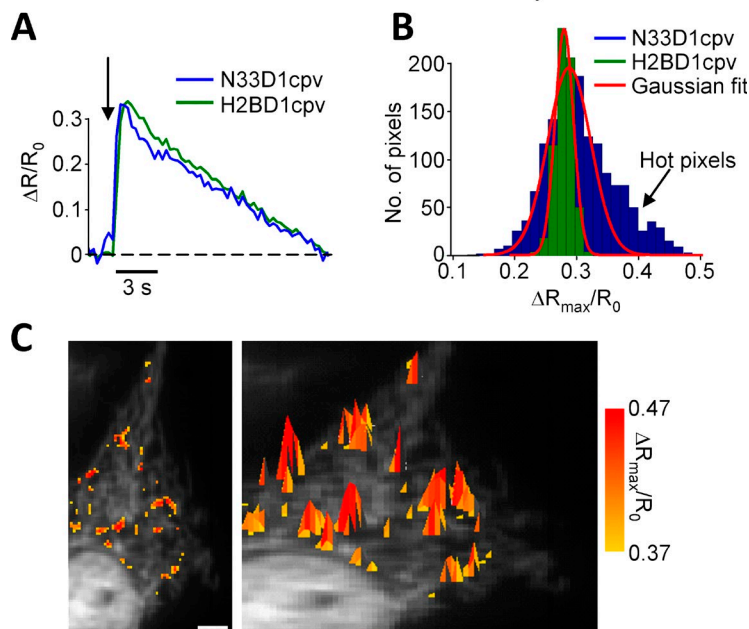
Figure 8. Mitochondrial \text{Ca}^{2+} hotspots. Pixel by pixel correlation showing the presence of \text{Ca}^{2+} microdomains on mitochondrial outer membrane (OMM) upon stimulation. HeLa cells cotransfected with nuclear (H2BD1cpv)- and OMM (N33D1cpv)-targeted Cameleons were treated with 100 \mu\text{M} histamine where indicated by the arrow in A. (A) The average [\text{Ca}^{2+}] rises, expressed as \Delta R/R_0 , of nucleus (green trace) and OMM (blue trace) are very similar. (B) The number and intensity of single pixels, expressed as \Delta R_{\text{max}}/R_0 of single pixels, of the nucleus (green) or OMM (blue) reached during the first 4 s after histamine stimulation were plotted. The Gaussian fit of the nuclear (green) and OMM (red) pixel distribution highlights the right tail caused by hot-spot formation on OMM upon cellular stimulation. (C) Yellow to red color representation of \Delta R_{\text{max}}/R_0 spatial distribution of pixels in 2D (left) and 3D (right), superimposed to YFP fluorescence image. Only pixels that during the 4 s after the histamine challenge have a \Delta R_{\text{max}}/R_0 exceeding by 125% the \Delta R/R_0 of the whole compartment were color coded. Bar, 5 \mu\text{m} (from Giacomello et al. [2010] with permission from Elsevier).
