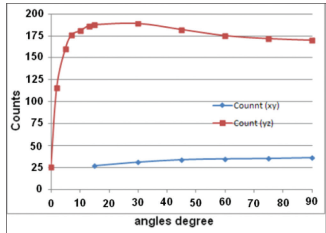
Figure 5: Sensitivity versus emission direction on xy and yz plane
