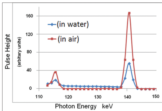
Figure 1: Pulse height distribution versus radiation photon energy in the air and water
