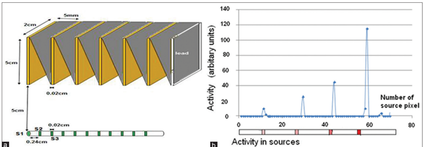
Figure 8: (a) Detector array with 36 vertical single side detector and (b) 71 source voxels with no equally activity
