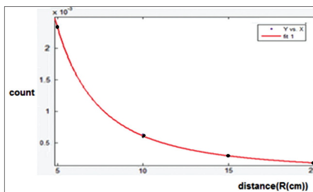
Figure 2: Detector counts versus source-detector distances
