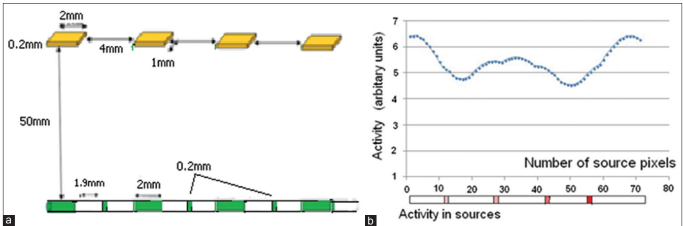
Figure 6: (a) Detector array with 36 horizontal detector and (b) 71 source voxels with different activity
