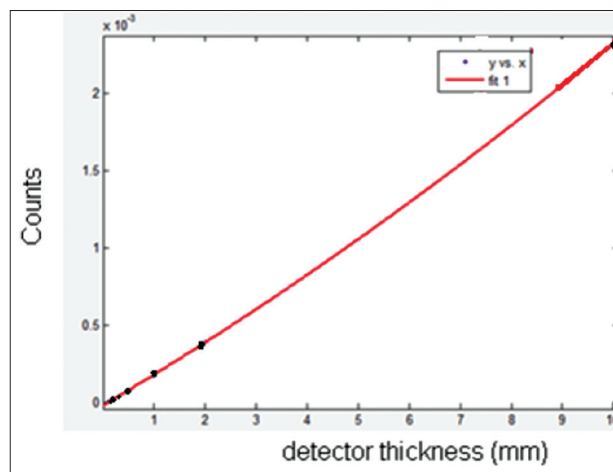
Figure 3: Detector sensitivity versus detector thickness
