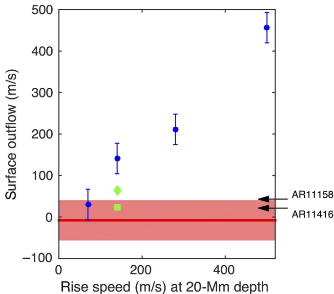
Fig. 4. Comparison of the azimuthal average of the horizontal surface outflow from HMI observations with the surface outflows seen in the simulations rules out flux tubes with total flux 10^{22} Mx rising with speeds above 140 m/s at 20-Mm depth. The simulations (blue circles) show a radial surface outflow that increases with the rise speed of the flux tube through the bottom boundary of the simulation domain. The error bars for the simulations show upper limits on the noise in the seismology measurement procedure. The horizontal black arrows show the observations for AR11416 and AR11158 (the examples shown in Fig. 3). The red shaded region shows the one- \sigma variations in the azimuthal average of the horizontal outflow at a distance of 15 Mm from the emergence location for the sample of 70 observed active regions. The green diamond shows the reduced field strength case (error bars not shown; the errors are the same as the other simulations), and the green square shows the reduced cross-section case. The simulations with a rise speed of 140 m/s with the tube located in the strongest upflow or strongest downflow at the bottom boundary produce diverging flows of about 90 m/s. As discussed in the text, the surface flows driven by flux emergence depend not only on the rise speed but also on the geometry and field strength of the rising flux tube.
