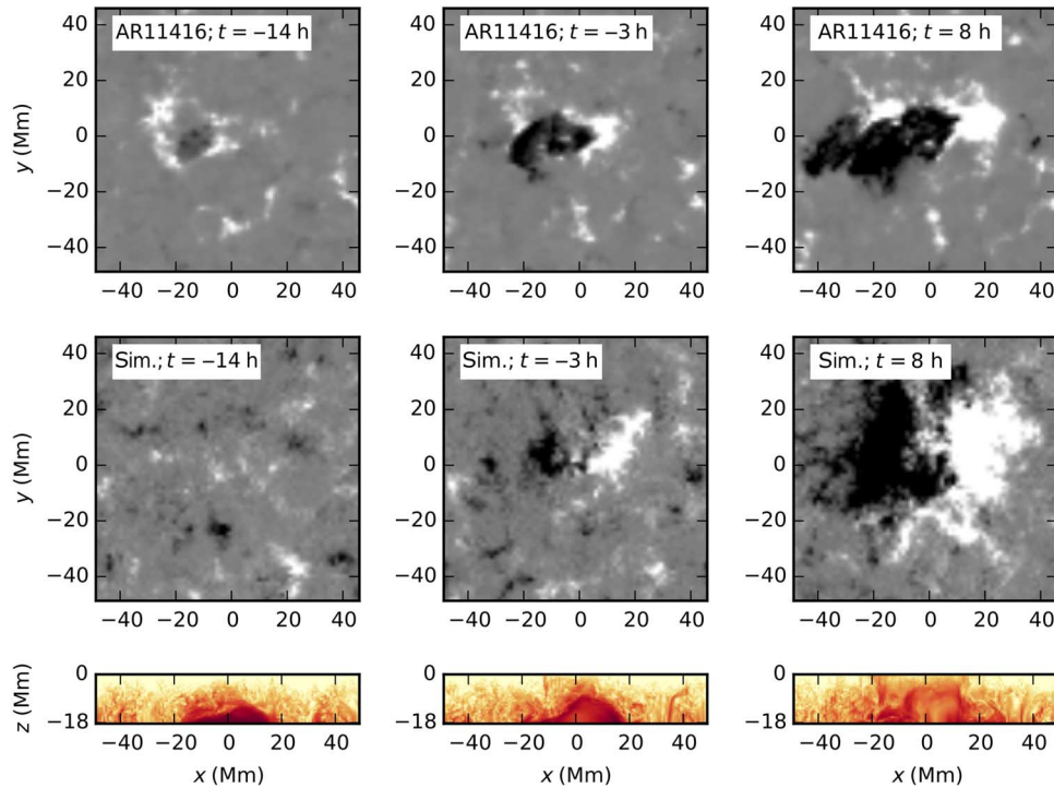
Fig. 2. Simulations of the emergence of magnetic flux through the photosphere reproduce many of the features of observed emergences. The top row shows, from left to right, the time evolution of the line-of-sight surface magnetic field associated with the emergence of AR11416 as seen by SDO/HMI. The images cover the time period from 14 hours before the emergence time to 8 hours after the emergence. The middle row shows the vertical surface magnetic field of a simulation for the case with a flux tube rising at a rise speed of 140 m/s. The bottom row shows vertical slices at y = 0 through the magnetic field strength in the same simulation. In the first two rows, positive (negative) line-of-sight magnetic field is shown in white (black). The gray scale is saturated at 120 G. In the bottom row, the color scale is the same as in Fig. 1.
