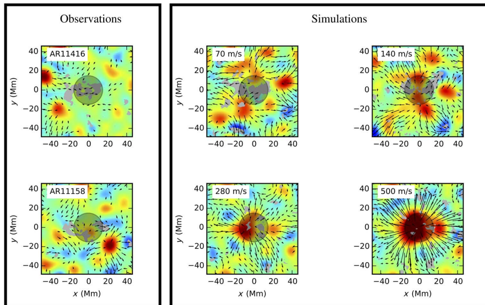
Fig. 3. At 3 hours before the emergence time, the near-surface flows inferred from HMI observations are dominated by convection, whereas the simulations show a diverging flow that increases in strength with the rise speed of the flux tube at 20-Mm depth. The two panels in the left column show maps of the horizontal divergence of the flows measured from helioseismology (red for diverging flows and blue for converging flows), flow maps from helioseismology (black arrows), and line-of-sight magnetic field strength (from magnetograms, shaded gray regions for fields stronger than 60 G) for the HMI observations of AR11416 and AR11158. The four-panel group on the right shows simulations for 10-kG flux tubes with rise speeds of 70, 140, 280, and 500 m/s at 20-Mm depth. The simulations with rise speeds of 280 and 500 m/s produce strong diverging flows that are not seen in the observations. The longest arrows represent flows of 400 m/s.
