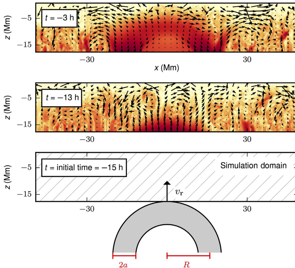
Fig. 1. Diagram of the setup for the simulation (bottom panel) and vertical slices through the simulation with a rise speed of 500 m/s at 13 and 3 hours before the emergence time (middle and top panels). In the bottom panel, the magnetic flux tube used to generate the bottom boundary condition is shown in gray. The major radius of the flux tube is given by R , the minor radius is given by a , and an untwisted magnetic field is oriented along the tube. Within the minor radius, the magnetic field has a Gaussian dependence of the form \exp[-2x^2/a^2] , where x is the distance from the center of the tube; the magnetic field is zero outside the tube. As the simulation progresses, the flux tube moves upward with rise speed v_r . In the top two panels, the log of the magnetic field strength is color-coded (red is the strongest field, and light yellow is the weakest), and the arrows show the flows in the plane of the vertical slice (the largest arrows represent about 3 km/s). Upward and horizontal diverging flows are apparent during the emergence process in this case.
