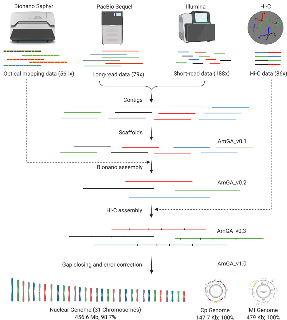
Fig. 2 Schematic of the de novo assembly of A. marina genome. Long-read and short-read data from PacBio Sequel and Illumina, respectively, were subjected to hybrid assembly to build contigs that were combined to build scaffolds. Super-scaffolds were built by combining the scaffolds from Bionano assembly and those from the previous step. Chromosome-scale assembly was built using the Hi-C chromosome conformation capture data, and the assembly was further refined by gap closing and error correction. Sequence data from a scaffold that contained the organellar genomes were re-assembled to build full-length circular chloroplast and mitochondrial genomes.
