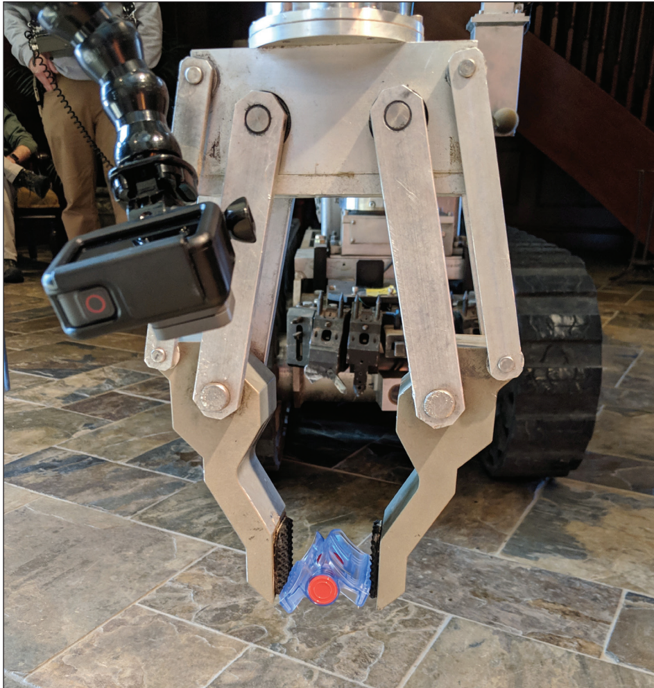
Fig. 3: Wolverine robot equipped with wound clamp in its manipulator.
