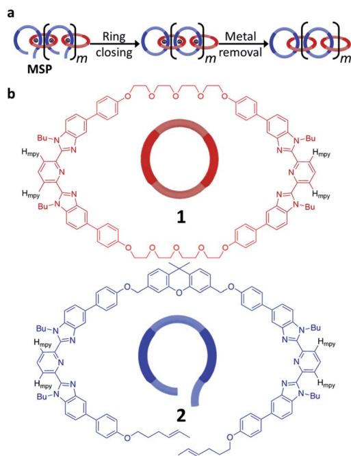
Fig. 2 (a) Poly[ n ]catenanes can be synthesized by assembly of a ditopic thread-like component (blue) and a ditopic macrocycle (red) via metal-templating to yield a metallocsupramolecular polymer (MSP). Ring closure of the blue component within the MSP followed by demetallation yields the poly[ n ]catenane. (b) Chemical structures and cartoon representations of the macrocyclic (1) and thread (2) components used in the synthesis of the poly[ n ]catenane. The 2,6-bis(benzimidazolyl)pyridine (Bip) component is darkened for identification and the m -pyridyl protons (H mppy ) are indicated in black.
