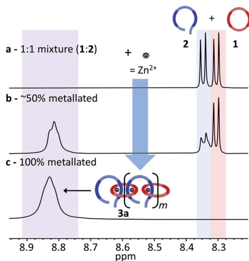
Fig. 4 The region of the ^1\text{H} NMR (500 MHz, 298 K) corresponding to the \text{H}_{\text{mppy}} protons peaks of (a) a 1 : 1 mixture of macrocycle 1 and thread 2 (in \text{CDCl}_3 ), (b) partial metallation of the mixture by titration of \text{Zn}(\text{NTf}_2)_2 (in \text{CD}_3\text{CN} ) and (c) the MSP 3a (in 1 : 5 \text{CD}_3\text{CN} : \text{CDCl}_3 , 20 mM w.r.t. 2 ).
