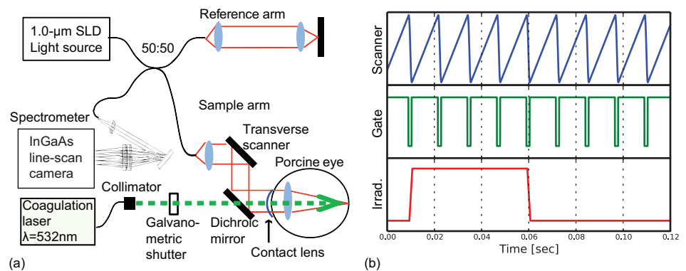
Fig 1. Experimental setup and timing chart. (a) Experimental setup. (b) Timing chart of the galvanometric scanner and image acquisition. Scanner, waveforms to scan the retina; Gate, a gate signal for OCT acquisition; Irrad., the coagulation laser output with an exposure time of 50 ms.
