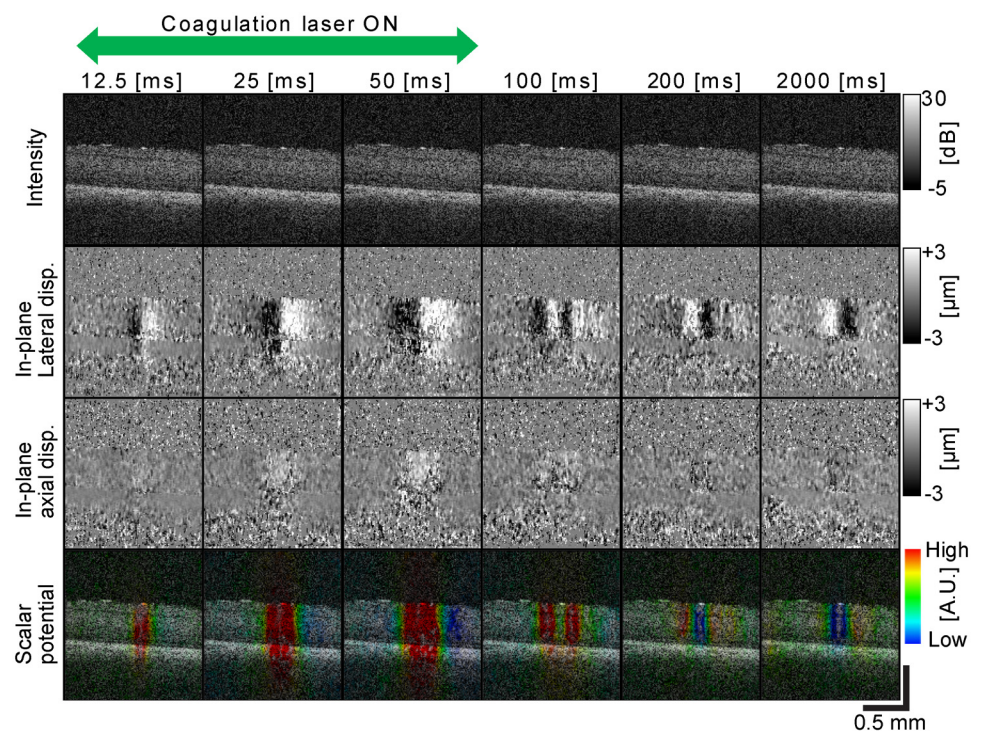
Fig 4. OCT B-scan images, in-plane lateral and axial displacements and scalar potentials at different time points (Class-1). OCT B-scan images (first row), in-plane lateral displacements (second row), in-plane axial displacements (third row), and the color composite images (fourth row) where the color represents the scalar potential at different time points.
