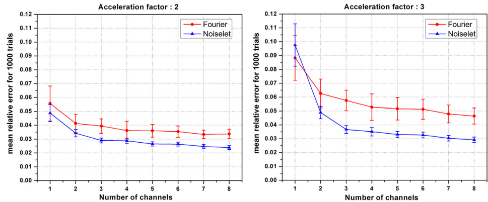
Fig 6. The mean relative error and standard deviation (vertical bar) versus the number of receive channels for acceleration factors of 2 and 3, showing that the error increases as the number of channels decreases. Noiselet encoding outperforms Fourier encoding for both acceleration factors when the number of channels is more than two. However for a single channel, noiselet encoding outperforms Fourier encoding only for the acceleration factor of 2.
