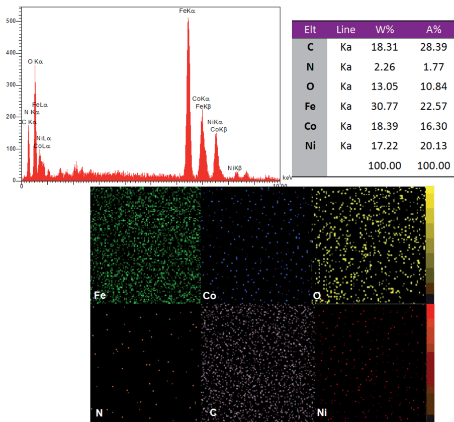
Fig. 4 EDX spectrum and elemental mapping of \text{CoFe}_2\text{O}_4@\text{GO}-\text{K} 22 \cdot \text{Ni} nanocomposite.
