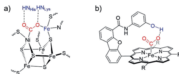
Figure 1. (a) [NiFe] carbon monoxide dehydrogenase active site [9] and (b) synthetic Fe-porphyrin [10] with bound \text{CO}_2 (in red) stabilized by outer coordination sphere interactions (in blue).
