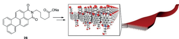
Figure 14. Self-assembled chromophores resulting in a polymer hydrogel. Adapted with permission from ref. [43a]. Copyright (2014) Springer Nature.
