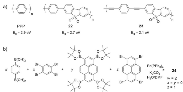
Figure 12. Tuning the band gap in (a) linear and (b) 3D microporous CPs.
