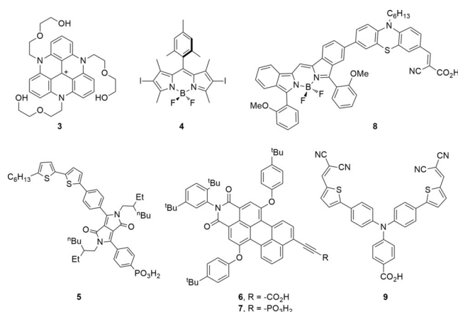
Figure 4. Organic PSs used in photocatalytic fuel synthesis.
