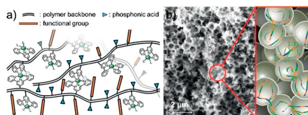
Figure 10. (a) Schematic representation of 16 and 17 . (b) Scanning electron microscopy image of inverse opal TiO 2 and schematic of polymer chains embedded in the porous scaffold. Reprinted with permission from ref. [36e]. Copyright (2019) John Wiley and Sons.
