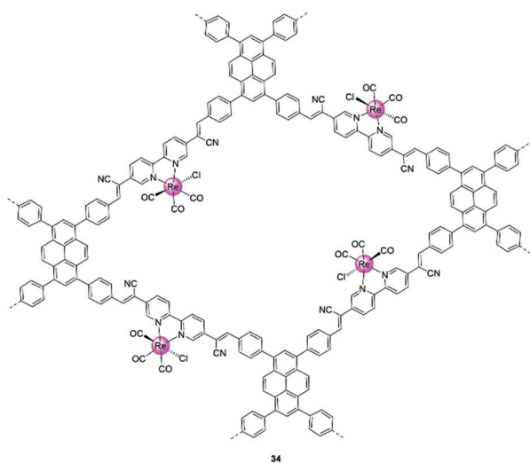
Figure 17. COF for photocatalytic \text{CO}_2 -to-CO conversion. [55]
