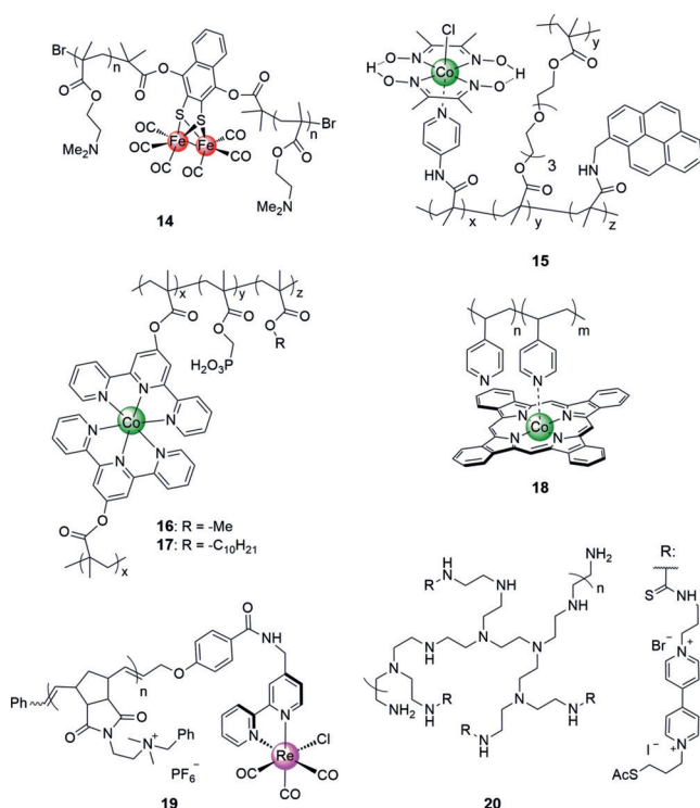
Figure 9. Scaffolding polymers for electrocatalytic systems.
