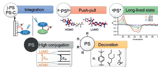
Figure 3. Examples of properties implemented in chromophores for optimizing photocatalytic performance (C = catalyst). Adapted with permission from ref. [19] and [20]. Copyright (2011 and 2018) Elsevier and American Chemical Society.
