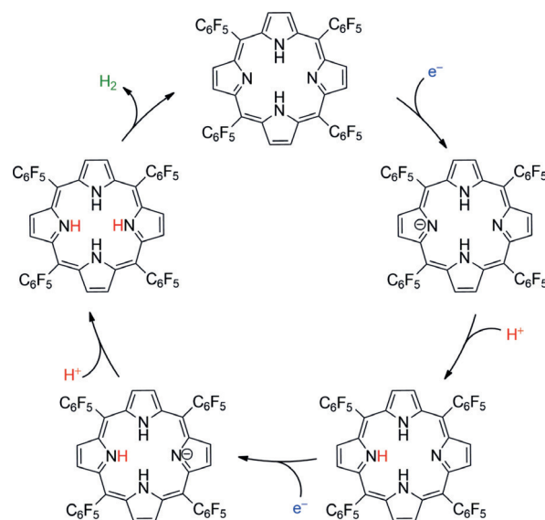
Figure 8. Proposed H 2 evolution mechanism for 12 . [32]
