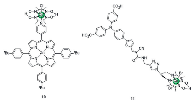
Figure 6. Photocatalysts for H 2 production based on transition metal-free PSs.
