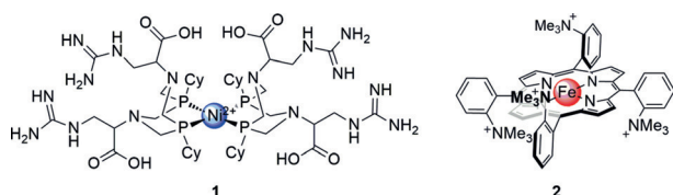
Figure 2. Catalysts with engineered ligands to stabilize reaction intermediates via secondary coordination sphere interactions. The functional groups in 1 are drawn as neutral for simplicity, but this may not reflect the real protonation state.
