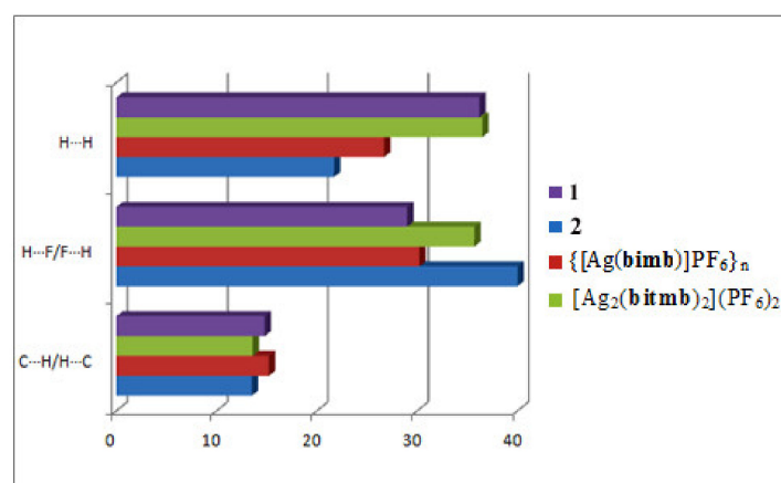
Figure 8. Estimated (%) contributions of selected intermolecular contacts to the Hirshfeld surface area for 1 and a series of \text{Ag}(\text{I}) complexes with \text{PF}_6^- .
