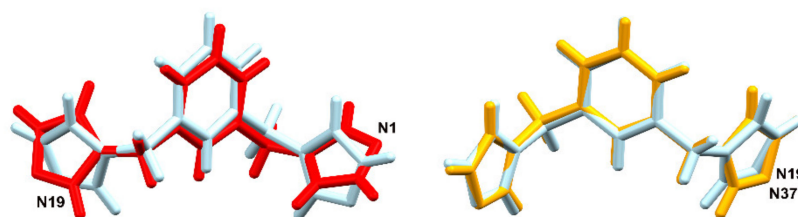
Figure 3. (On the left) overlay of the ligands containing N1 (red) and N19 (blue), (the RMS deviation after inversion is 0.9108 Å); and (on the right) overlay of the ligands containing N37 (orange) and N19 (blue), (the RMS deviation is 0.1832 Å) in 1 .
