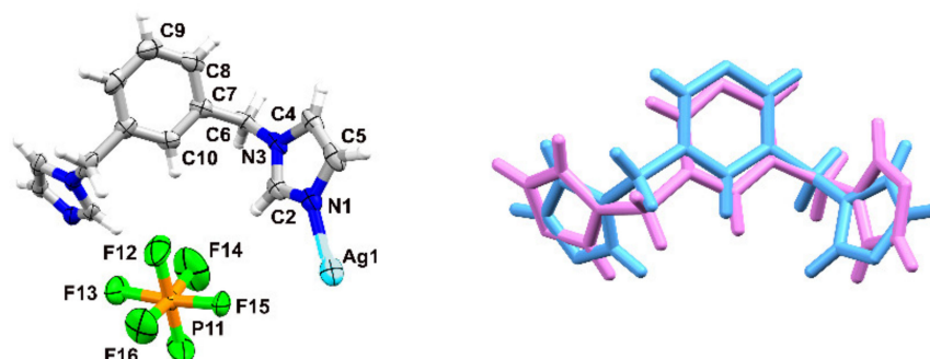
Figure 6. (On the left) a fragment of the helical chain in 2 , with the atomic displacement plot shown at 50% probability; unlabeled ligand atoms are generated by the symmetry operation x, \frac{1}{2} - y, 3/2 - z ; for the counterion: 3/2 - x, 1 - y, z ; (on the right) overlay of 2 (blue) with the ligand present in the related Ag(I) complex with bimb (magenta, methyl group removed for clarity); the RMS deviation is 1.0325 Å.
