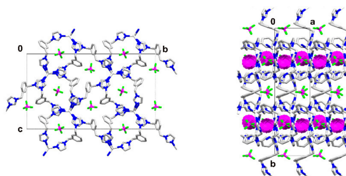
Figure 5. (On the left) packing diagram of 1 shown down the a axis; (on the right) packing diagram shown down the c axis exposing the voids (in pink) present between counterions; hydrogen atoms omitted for clarity.
