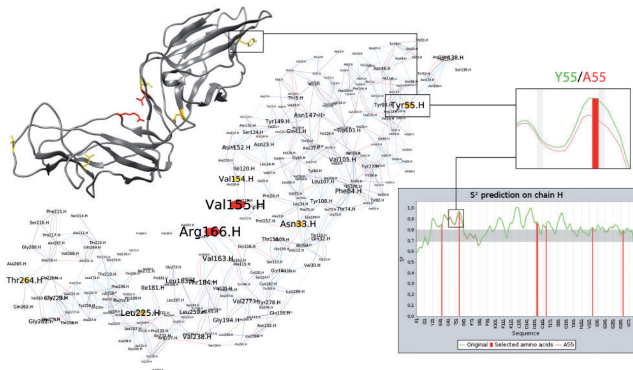
Fig. 1. Example of RINspector inter-module connectivity. Central residues are colored from yellow ( Z -score = 2) to red ( Z -score \geq 4 ) on structure and network. The central residues are indicated with red bars in the flexibility graph. The zoom shows the increase in local flexibility for the Y55A mutation (green to red curve)
