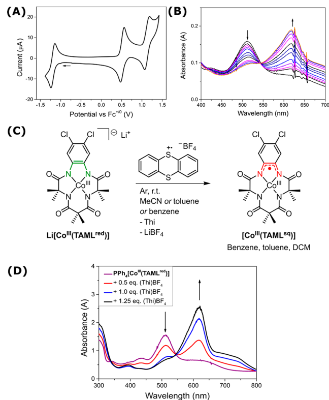
Scheme 3. (A) Cyclic Voltammogram of PPh 4 [Co III (TAML red )] in DCM (Details in the SI), (B) UV-vis-SEC Oxidation of PPh 4 [Co III (TAML red )] in DCM (Details in the SI), (C) Oxidation of [Co III (TAML red )] - to [Co III (TAML sq )] with (Thi)BF 4 , and (D) UV-vis Titration of PPh 4 [Co III (TAML red )] in DCM (0.15 mM) with Increasing Amounts of (Thi)BF 4
