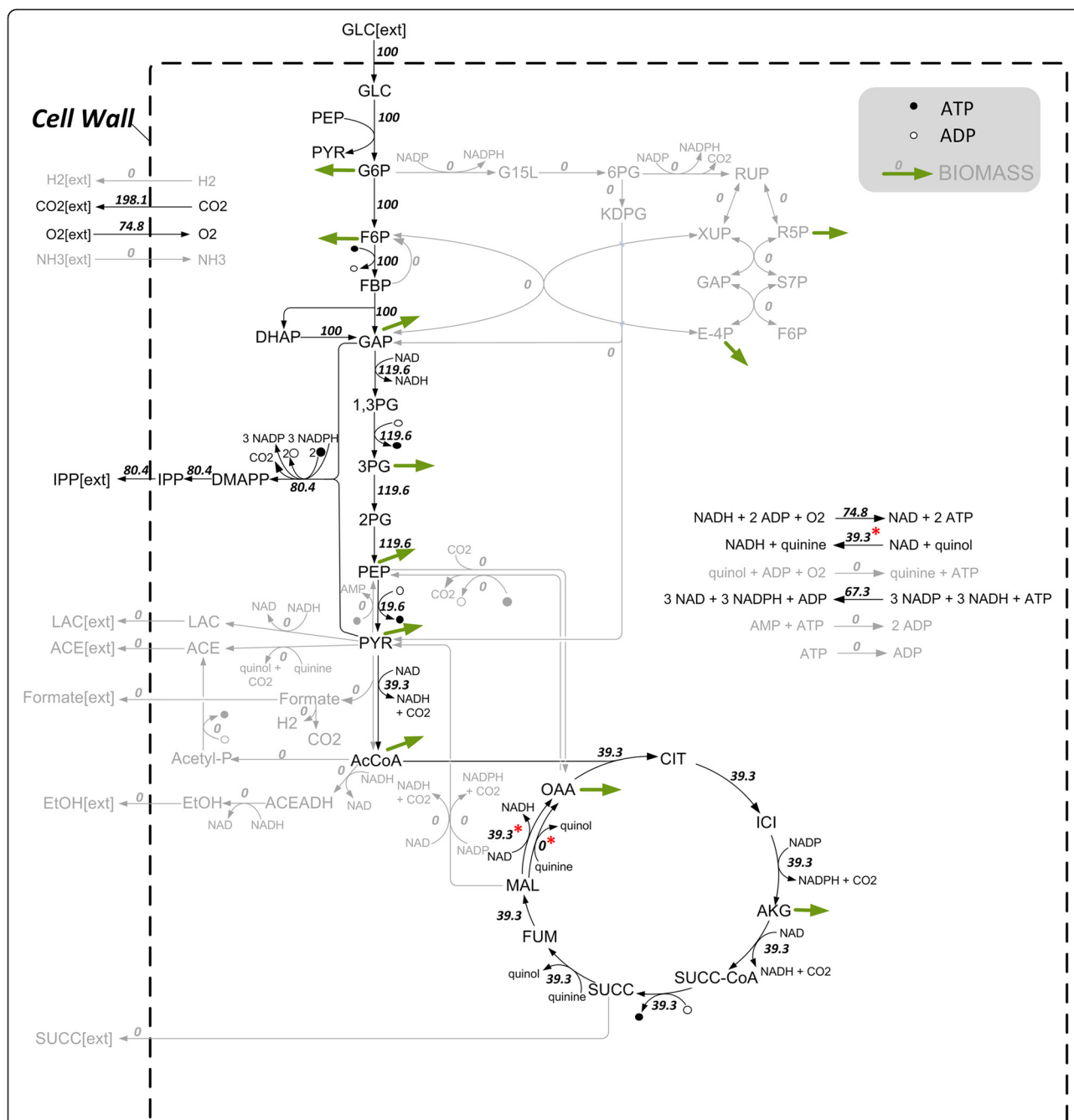
Figure 3 Optimal flux distribution of E. coli . Wild type (DXP pathway) on glucose as single carbon source without biomass formation (one of two modes with maximum theoretical IPP carbon yield). Numbers indicate relative molar fluxes (mmol/(gCDW h), CDW = cell dry weight) normalized to glucose uptake. Grey reactions are not active (flux = 0). Variable fluxes within two optimal modes are marked with an asterisk (*). Bold green arrows indicate biomass precursors.
