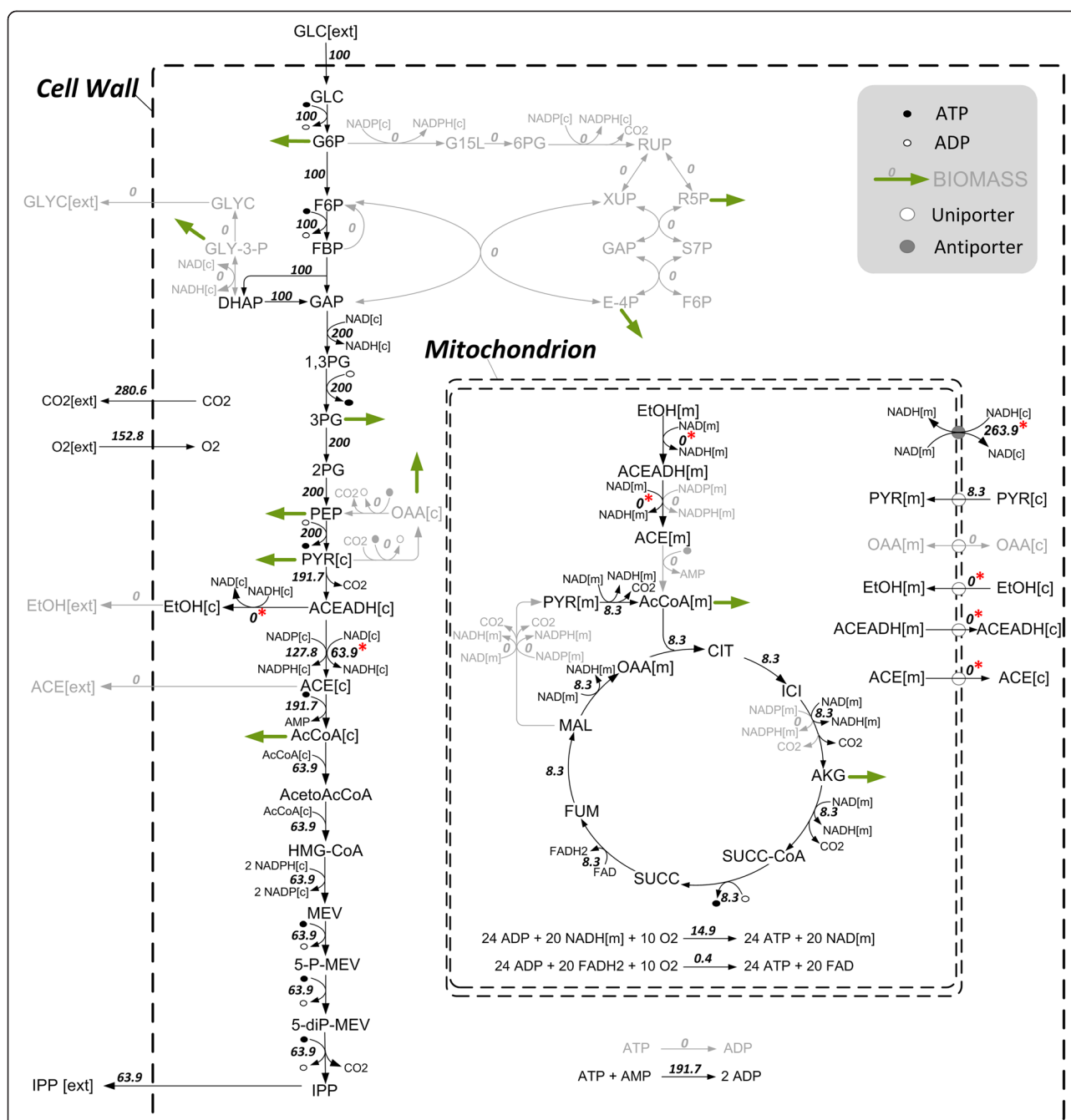
Figure 4 Optimal flux distribution of S. cerevisiae . Wild type (MVA pathway) on glucose as single carbon source without biomass formation (one out of five modes with maximum theoretical IPP carbon yield). Numbers indicate relative molar fluxes (mmol/(gCDW h), CDW = cell dry weight) normalized to glucose uptake. Grey reactions are not active (flux = 0). Variable fluxes within the 5 optimal modes are marked with an asterisk (*). Bold green arrows indicate biomass precursors.
