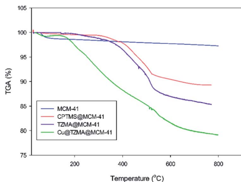
Fig. 7 TGA curves of MCM-41, CPTMS@MCM-41, TZMA@MCM-4 and Cu@TZMA@MCM-41.
