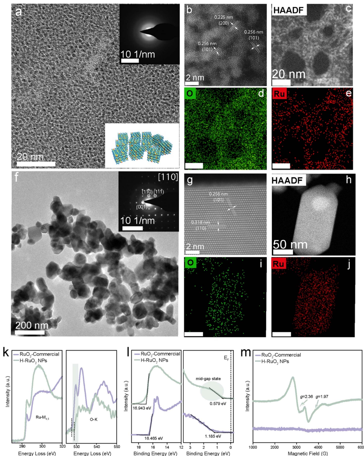
Fig. 2 Structural and compositional characterization of commercial and H-RuO 2 NPs. (a) TEM image of H-RuO 2 (inset shows the corresponding SAED pattern showing an amorphous nature). (b and c) HAADF-STEM images of H-RuO 2 at high (collected after a beam shower) and low magnifications. (d and e) EDX elemental mapping of H-RuO 2 . (f) TEM image of commercial RuO 2 (inset displays the corresponding SAED pattern). (g and h) HAADF-STEM images of commercial RuO 2 at atomistic and low magnifications. (i and j) EDX elemental mapping of commercial RuO 2 . (k) EELS spectra of the Ru-M 4,5 edge (left) and EELS spectra of the O-K edge (right) for commercial and H-RuO 2 . (l) Photoemission cutoff (left) and valence band (right) UPS spectra of commercial and H-RuO 2 . (m) EPR spectra of commercial and H-RuO 2 .
