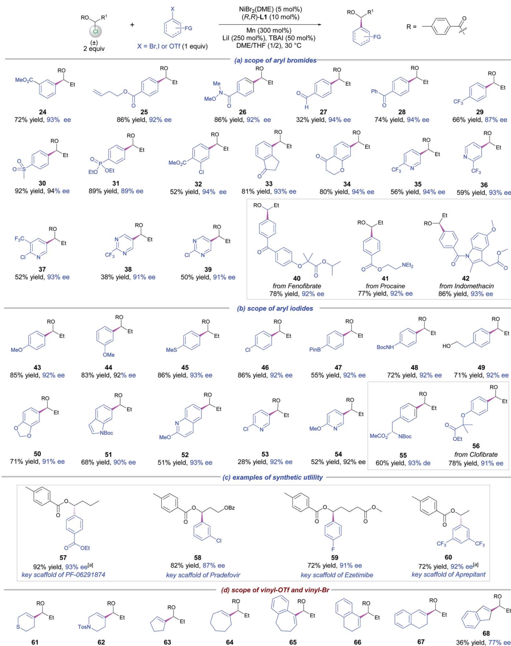
Scheme 3 Scope of aryl/vinyl electrophiles. Reactions conducted on a 0.15 mmol scale for 40 h, ee was determined by chiral HPLC analysis. [a] ( S,S )-L1 used as the chiral ligand. [b] With vinyl-OTf. [c] With vinyl-Br.
