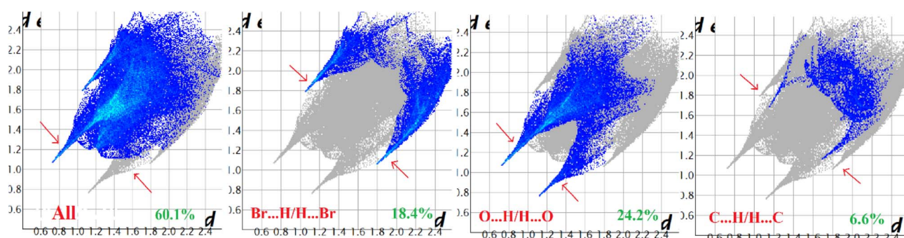
Fig. 8 Fingerprint plot of complex 1: full and resolved into Br...H/H...Br, O...H/H...O, and C...H/H...C contacts contributed to the total Hirshfeld surface area.
